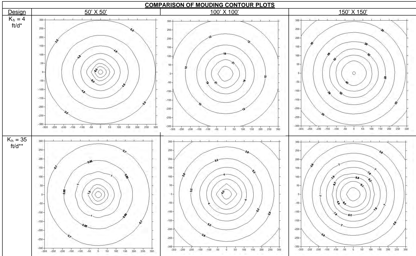
Figure 1. Comparison of Mounding as a Function of Design and Hydraulic Conductivity
