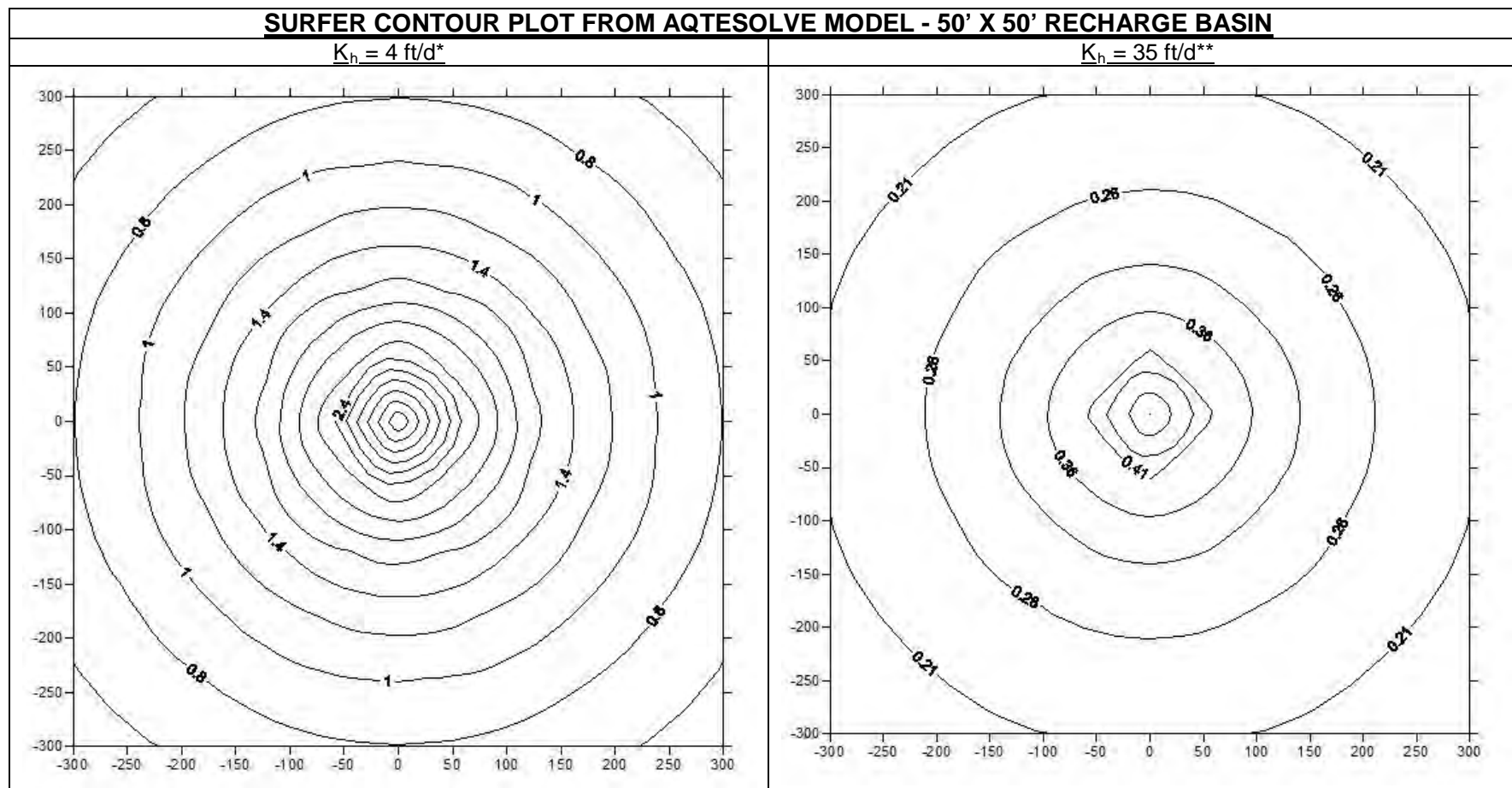
Figure 2. Contour Plots of Mounding up to 300 ft. away from the Center of the Soil Flushing System for the 50' X 50' Design Infiltration Rate of 0.27 ft/day
