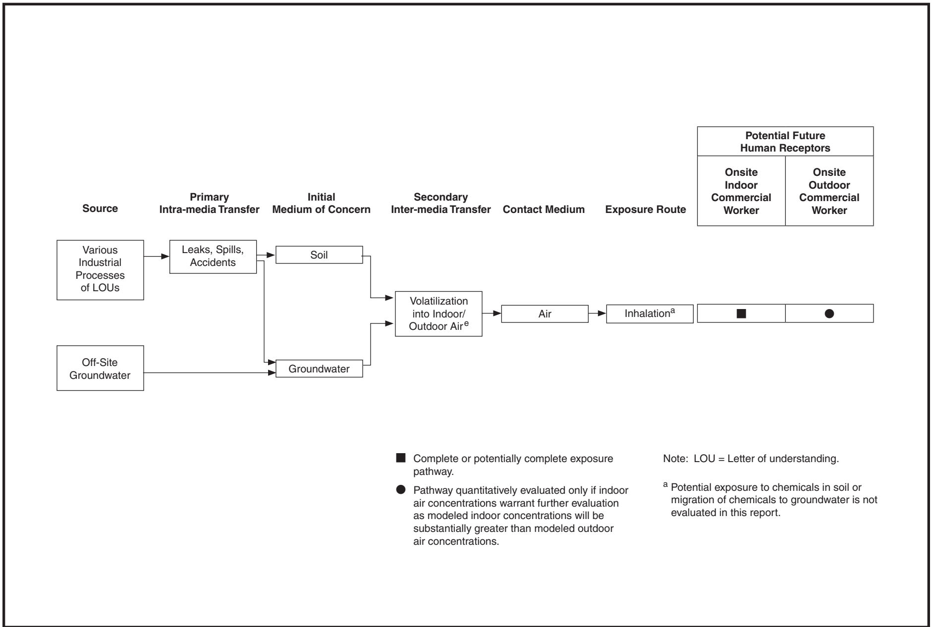
Figure 3. Conceptual site model diagram for potential human exposures to chemicals in soil gas, Tronox Facility, Henderson, Nevada a
