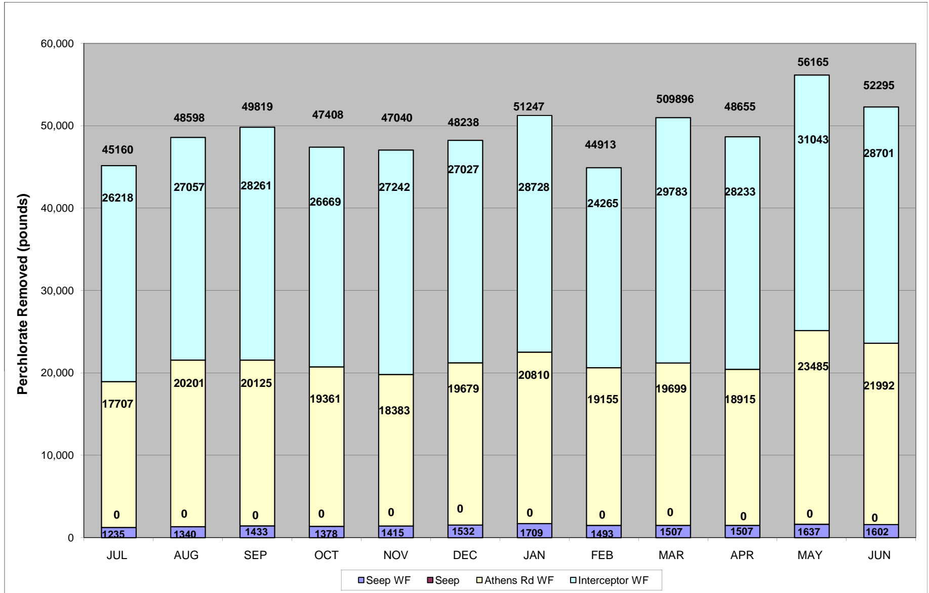
FIGURE 9 PERCHLORATE REMOVED FROM THE ENVIRONMENT JULY 2009 TO JUNE 2010
