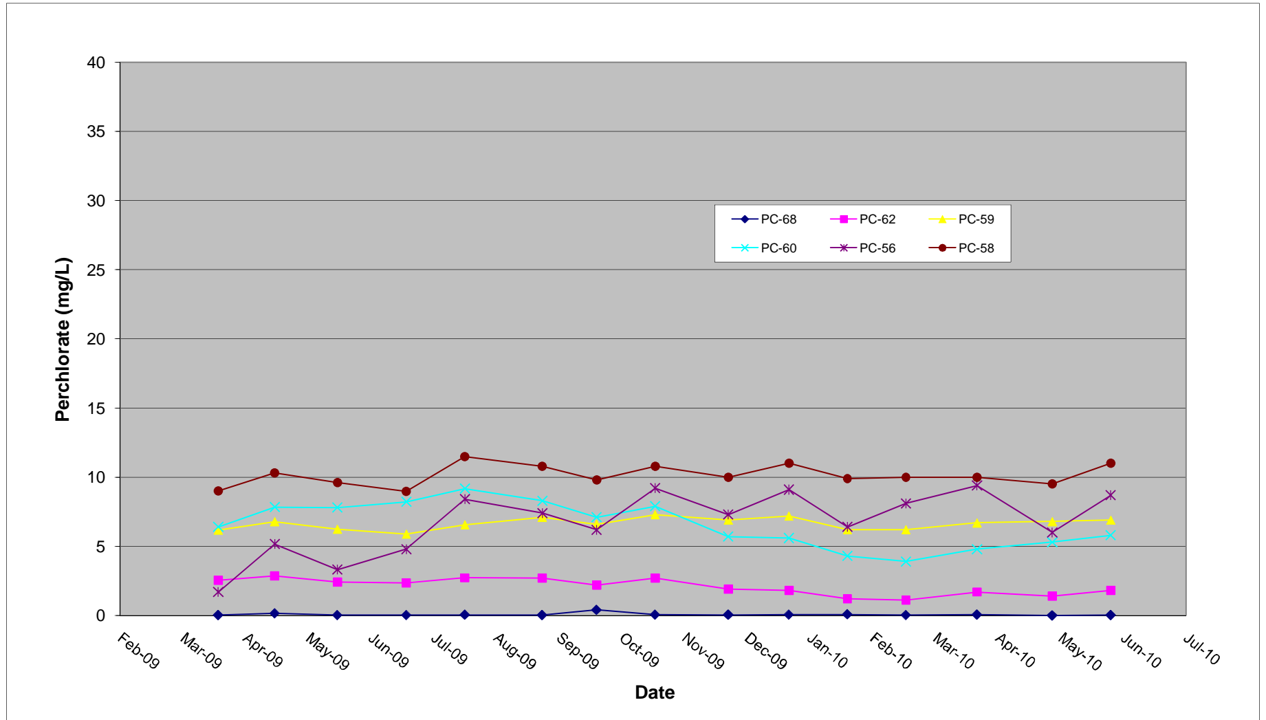
FIGURE 25A LOWER PONDS WELL LINE PERCHLORATE CONCENTRATION TREND GRAPH APRIL 2009 TO JUNE 2010
