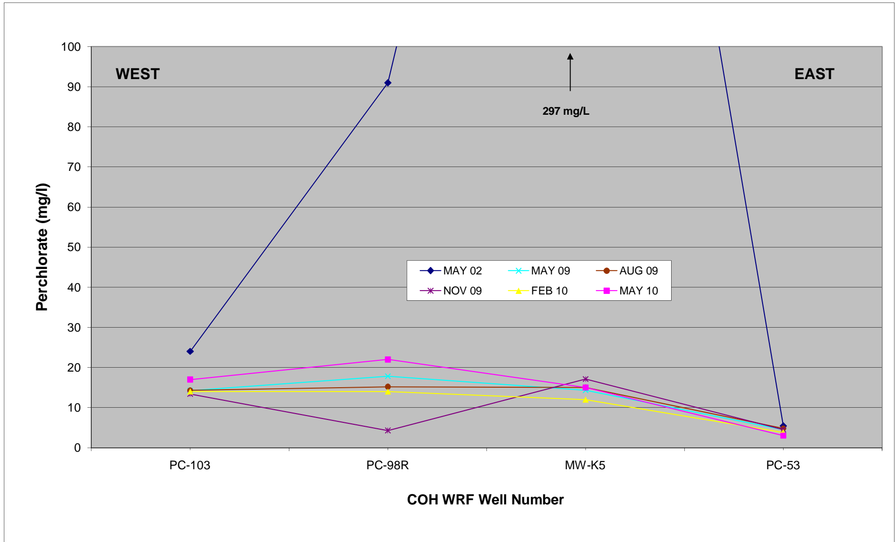
FIGURE 22 CITY OF HENDERSON WRF WELL LINE PERCHLORATE CONCENTRATION TREND GRAPH
