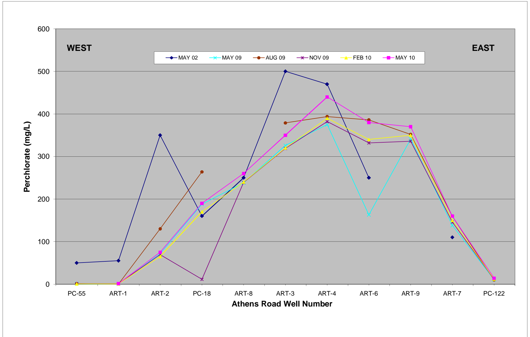
FIGURE 16 ATHENS ROAD WELL FIELD PERCHLORATE CONCENTRATION TREND GRAPH
