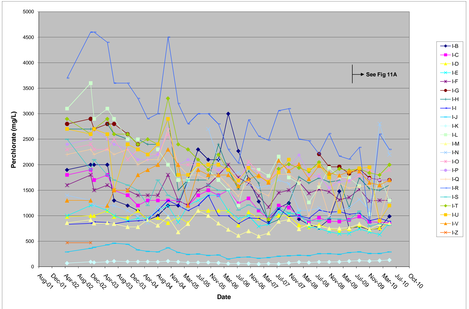
FIGURE 11 INTERCEPTOR WELL FIELD PERCHLORATE CONCENTRATION TREND GRAPH
