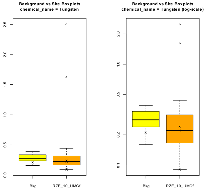
RZE – Background Data (10-UMCf fbg), Site Data (10-UMCf fbg)
