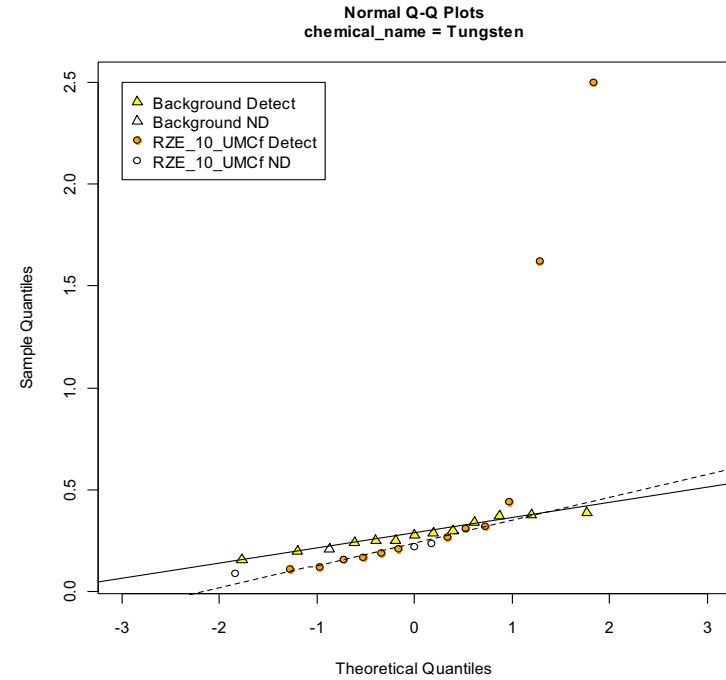
RZE – Background Data (10-UMCf fbg), Site Data (10-UMCf fbg)
