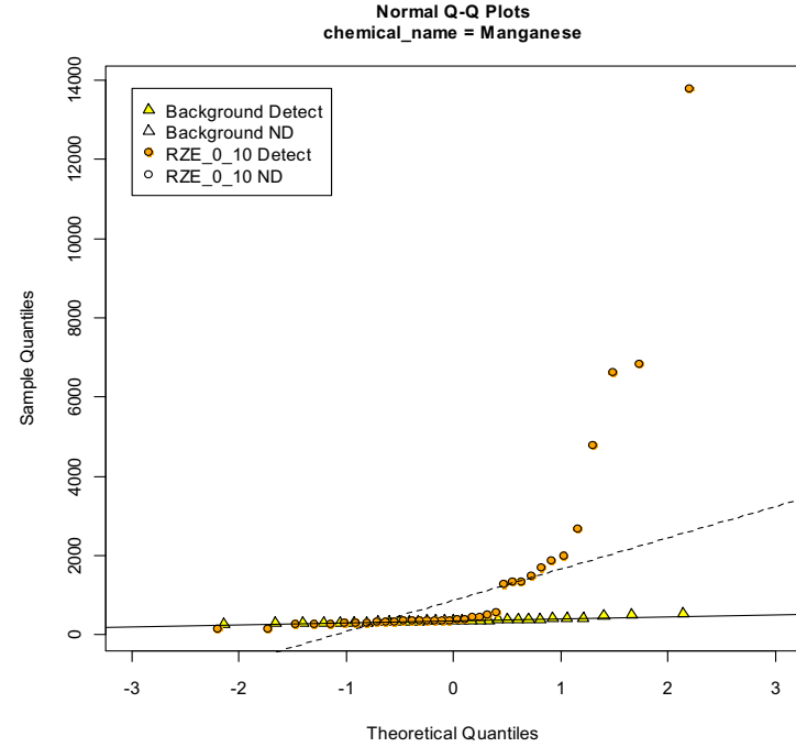
RZE – Background Data (0-10 fbs), Site Data (0-10 fbs)
