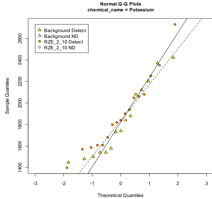
RZE – Background Data (2-10 fbgs), Site Data (2-10 fbgs)
