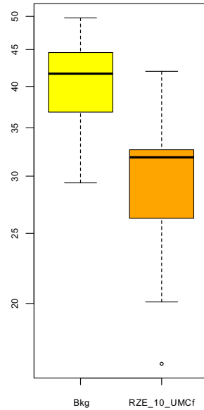
Background vs Site Boxplots chemical_name = Vanadium (log-scale)
