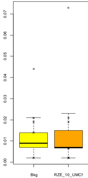
Background vs Site Boxplots chemical_name = Mercury
