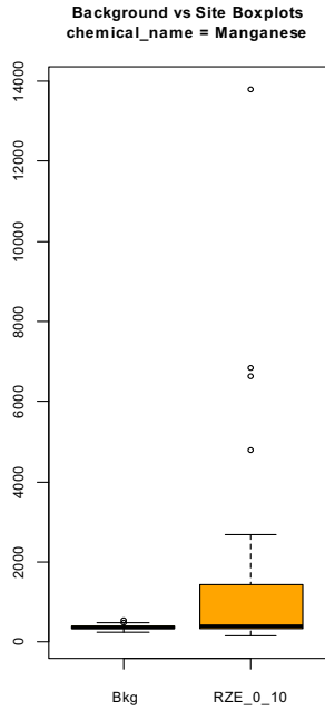
RZE – Background Data (0-10 fbs), Site Data (0-10 fbs)
