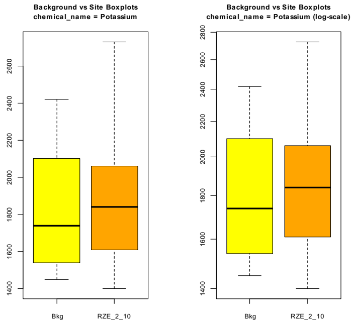
RZE – Background Data (2-10 fbgs), Site Data (2-10 fbgs)
