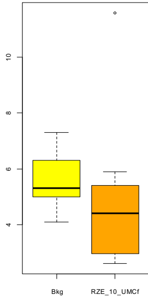
Background vs Site Boxplots chemical_name = Cobalt
