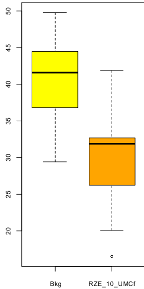
Background vs Site Boxplots chemical_name = Vanadium
