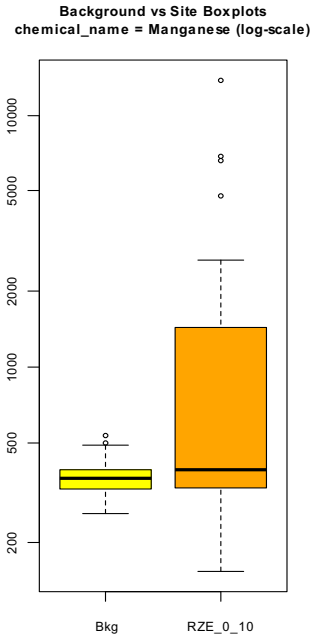
RZE – Background Data (0-10 fbs), Site Data (0-10 fbs)
