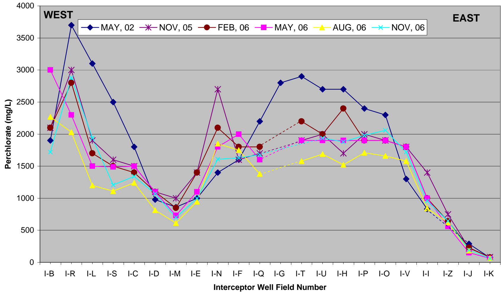
FIGURE 9: INTERCEPTOR WELL FIELD PERCHLORATE SECTION GRAPH TRONOX LLC HENDERSON, NEVADA
