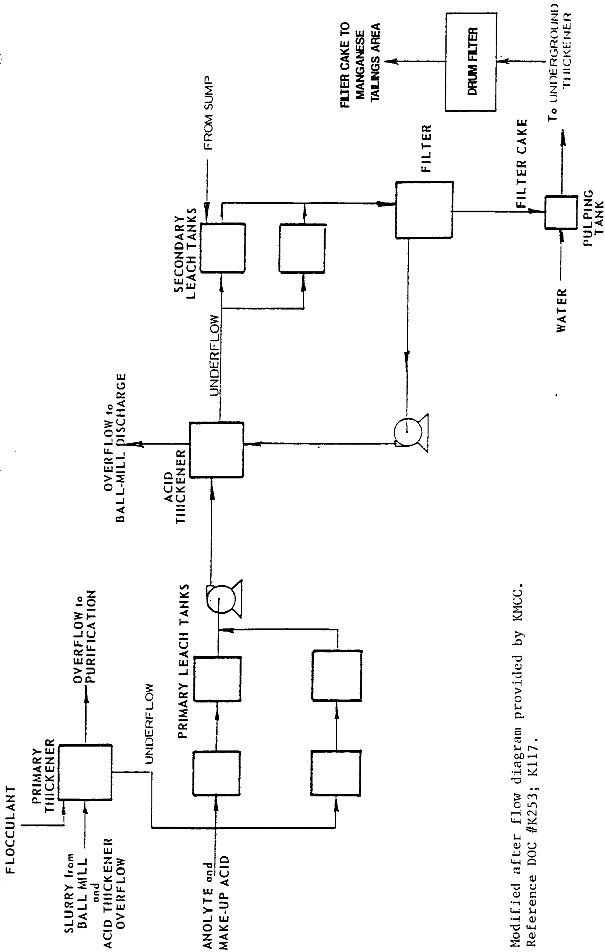
FIGURE 4.9.2 MANGANESE DIOXIDE LEACH PLANT PROCESS (LEACHING PORTION) FLOW DIAGRAM
