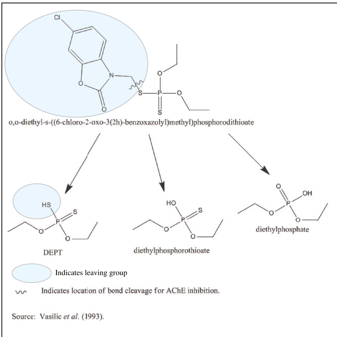
Figure 4. Metabolic Origin of DEPT from o,o -diethyl- s -((6-chloro-2-oxo-3(2 h )-benzoxazolyl)methyl)phosphorodithioate (Phosalone).
