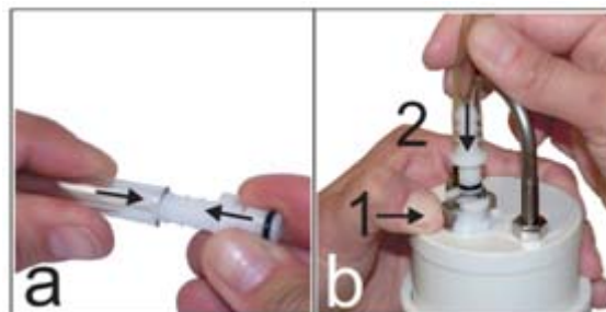
Fig. 14. Connecting the Quick Connection to the RU.
