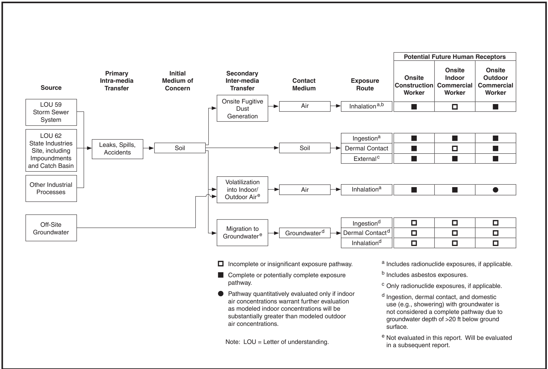
Figure 4. Conceptual site model diagram for potential human exposures—Remediation Zone A, Tronox Facility, Henderson, Nevada
