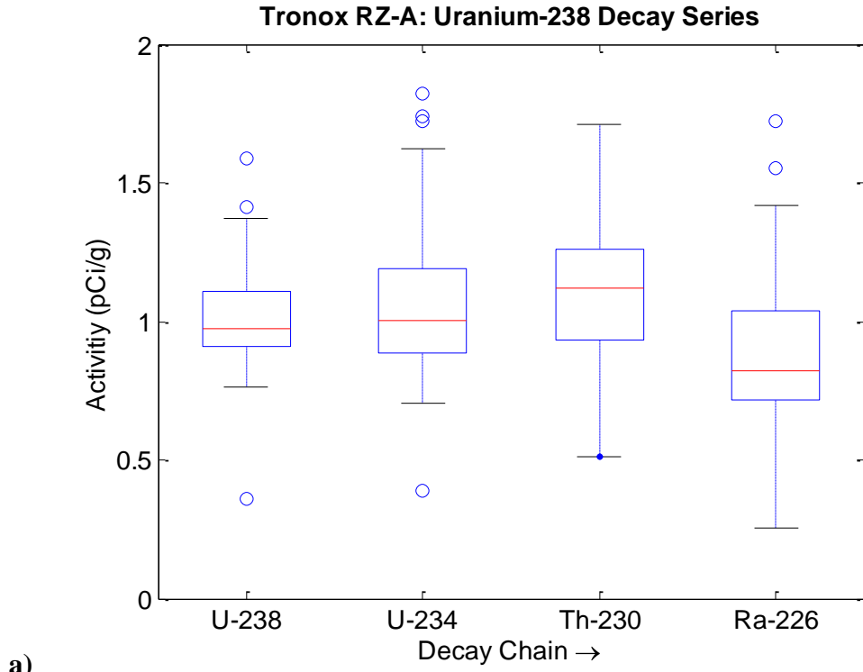
FIGURE 5 RZ-A Box-and-Whisker Diagrams for Thorium-232 and Uranium-238 Decay Series
