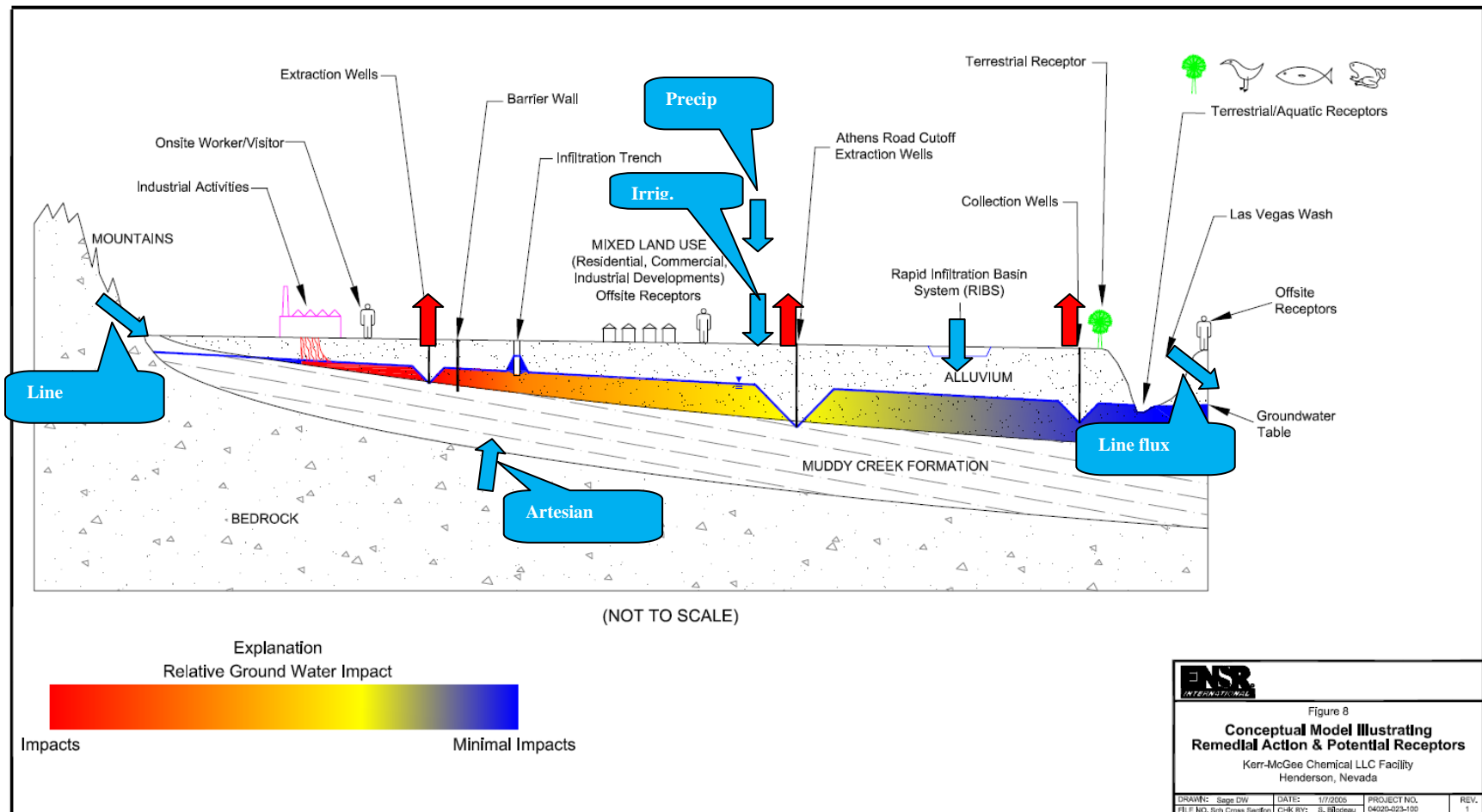
Figure 3 – Preliminary Conceptual Site Model Drawing (from ENSR, 2005)
