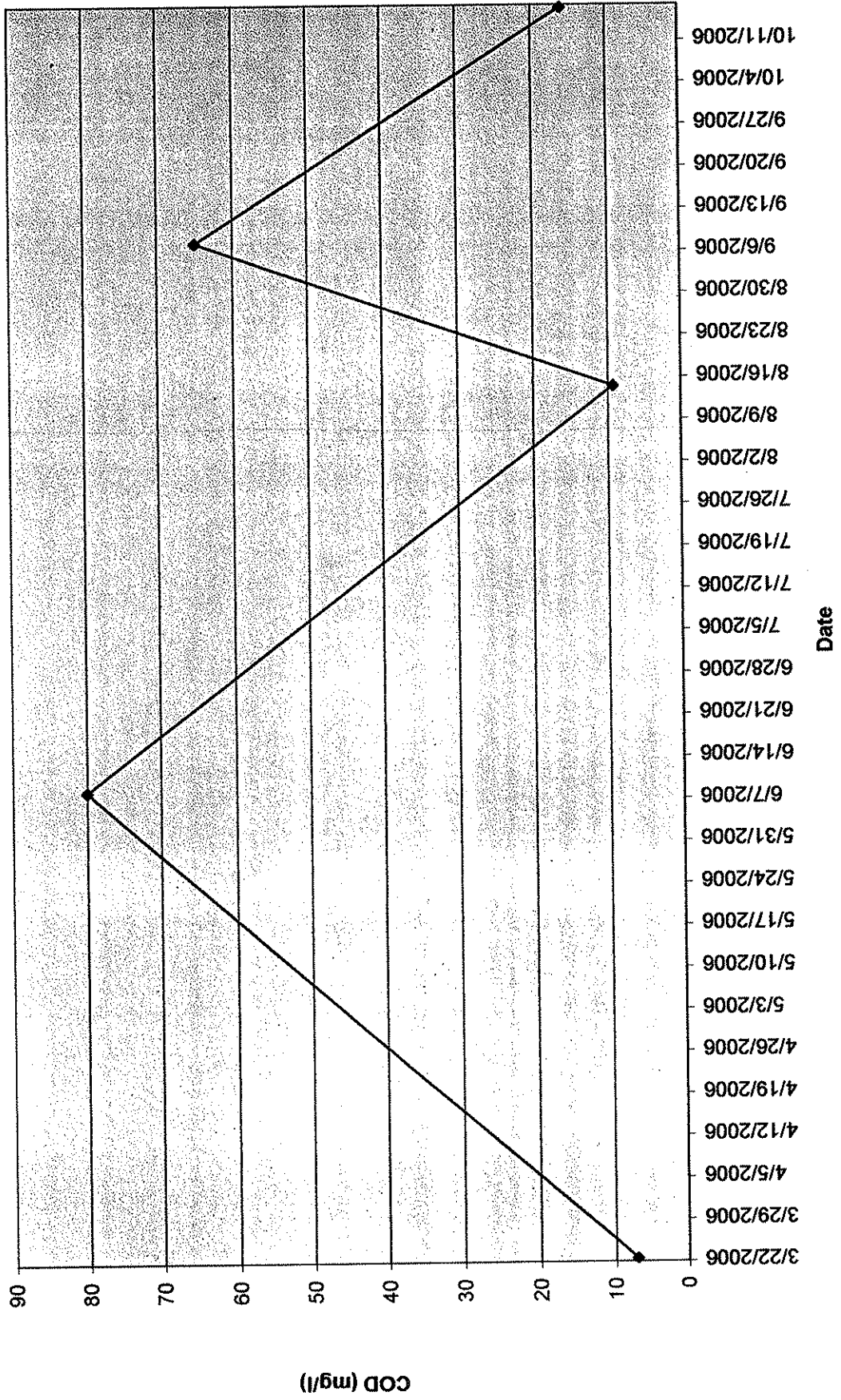
2006 - Outfall 002 COD Concentration - Storm and Non-Storm
