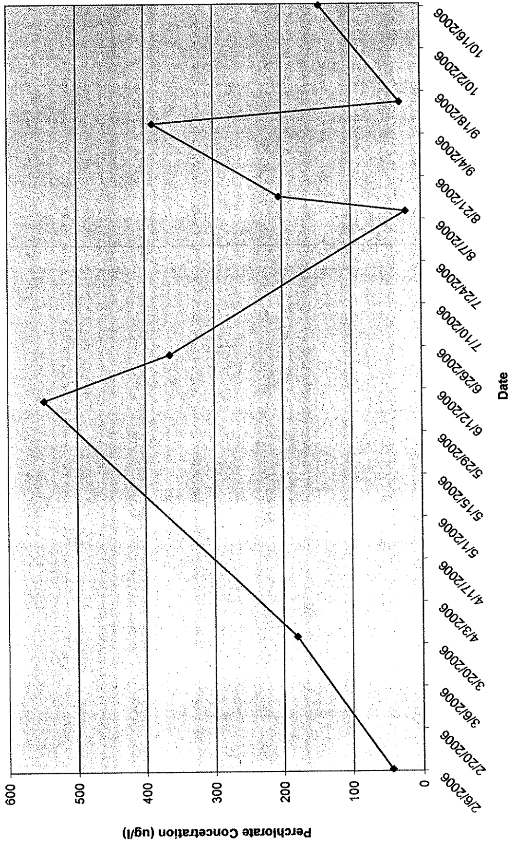
2006 - Outfall 001 Perchlorate Concentrations - Storm and Non-Storm
