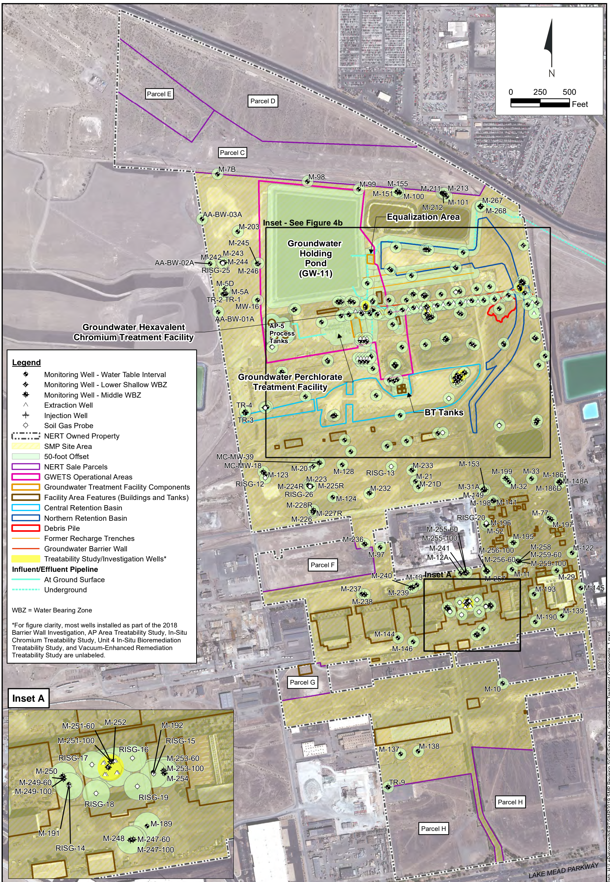
Existing On-Site GWETS Components & Monitoring and Injection Locations Nevada Environmental Response Trust Site, Henderson, Nevada Figure 4a
