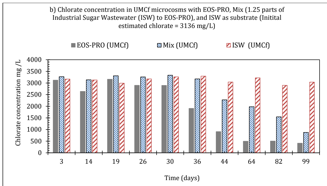
Figure 5.10: Concentration of chlorate in QAL (a) and UMCf (b) microcosms with EOS-PRO, Mix, and Industrial Sugar Wastewater as substrate
