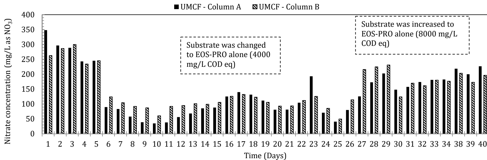
a. Effluent nitrate concentrations (mg/L as NO 3 ) concentrations in UMCF columns fed with high substrate-mixture of Industrial Sugar Wastewater and EOS-PRO (45880 mg/L COD eq) or EOS-PRO alone (4000 mg/L to 8000 mg/L COD eq) as substrate or no substrate
