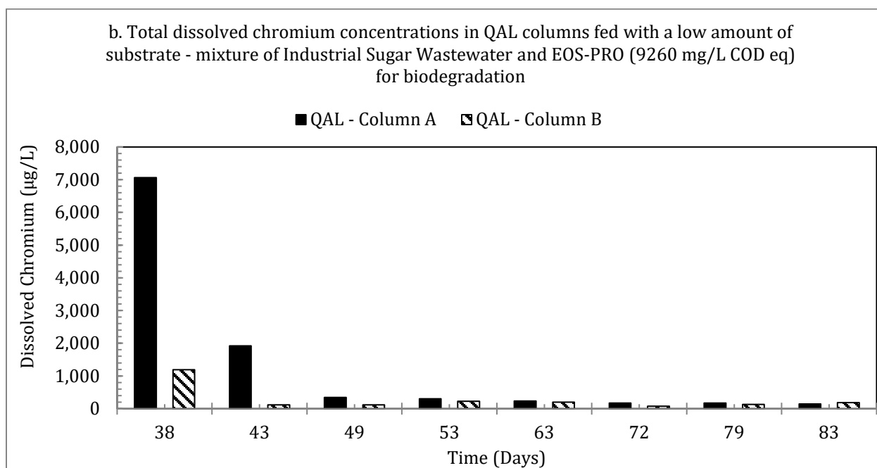
Figure 5.35: Total dissolved Chromium in the QAL columns fed with - a high amount of substrate (mixture of Industrial Sugar Wastewater at 7% and EOS-PRO at 2%), no substrate and EOS-PRO alone at 0.2% and 0.4% (a) and a low amount of substrate (mixture of Industrial Sugar Wastewater at 1.5% and EOS-PRO at 0.4%) (b).
