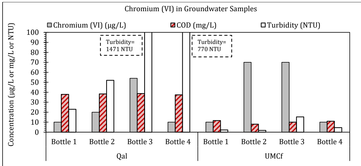
Figure 3.2: Hexavalent chromium, COD and Turbidity varied in each groundwater sample from UFIW-06 received on 7/22/2016 from both depths.
