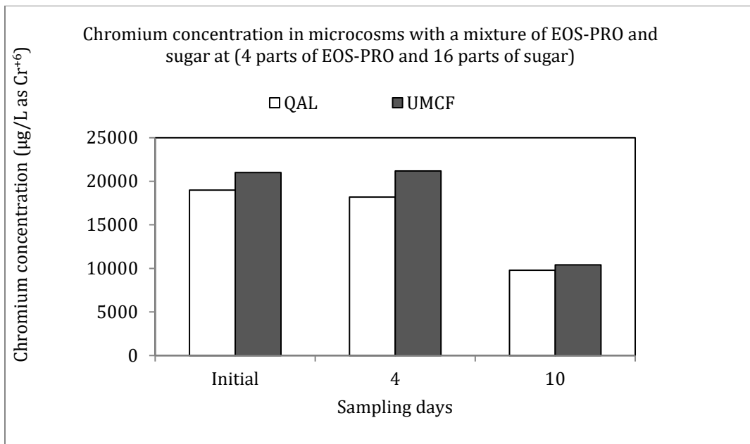
Figure 5.29: Cr (VI) in QAL and UMCf microcosms with a mixture of EOS-PRO and sugar as substrate.
