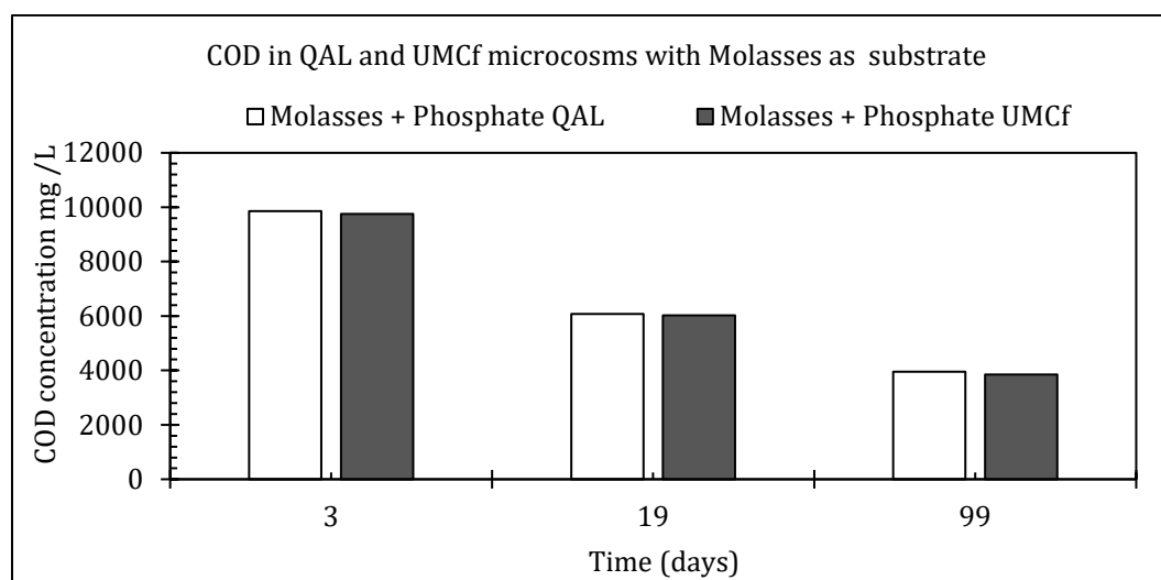
Figure 5.2: COD concentration in filtered samples in QAL and UMCf using Molasses with phosphate as substrate
