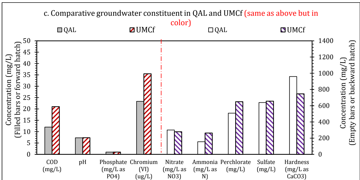
Figure 3.5: Groundwater from UFIW-03 received on 11/22/2016 for characterization in quaternary alluvial layer, QAL (25-30 ft) (a), muddy creek formation, UMCf (35-40 ft) (b), and comparison between QAL and UMCf (c)
