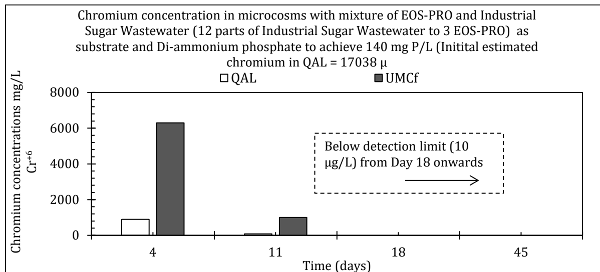
Figure 5.20: Cr (VI) concentrations in QAL and UMCf microcosms with a mixture of EOS-PRO and Industrial Sugar Wastewater as substrate.
