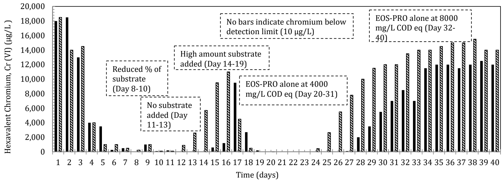
a. Effluent Cr (VI) concentrations in UMCf columns fed with a high amount of substrate- mixture of Industrial Sugar Wastewater and EOS-PRO (45880 mg/L COD eq) or EOS-PRO alone (4000 mg/L to 8000 mg/L COD eq) as substrate or no substrate
