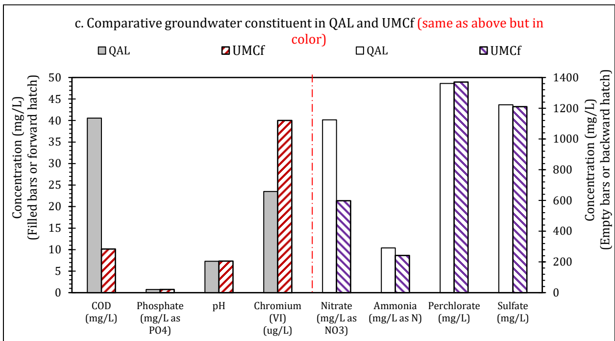
Figure 3.1: Groundwater characterization in quaternary alluvial layer (25-30 ft) (a), muddy creek formation (35-40 ft) (b) groundwater from UFIW-06 received on 7/22/2016 and comparison of QAL and UMCf groundwater (c). The contaminants concentrations for the filled and with forward hatched bars (left of the vertical dotted line) are read on the left y-axis and for the filled and with backward hatched bars (right of the vertical dotted line) are read on the right y-axis.
