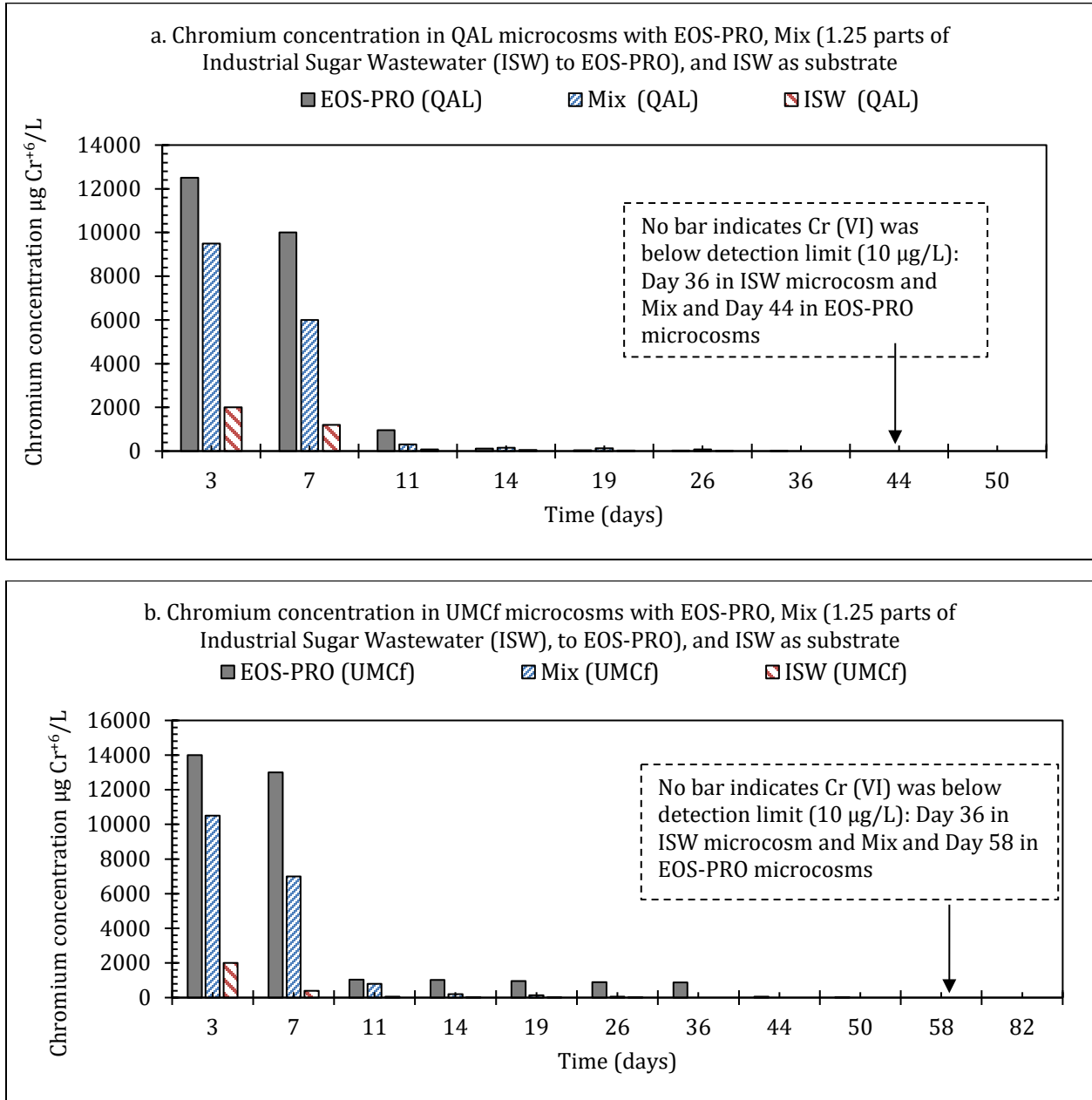
Figure 5.4: Cr (VI) in QAL (a) and UMCf (b) microcosms with EOS-PRO, Mix, and Industrial Sugar Wastewater as substrate.
