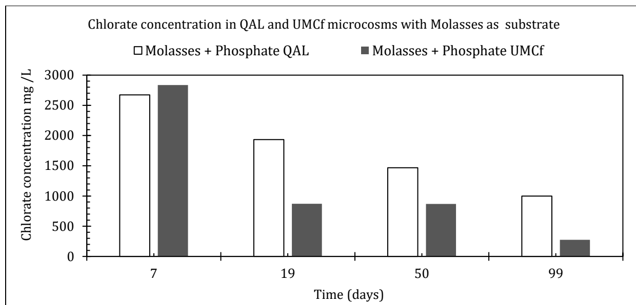
Figure 5.11: Chlorate concentration in QAL and UMCf microcosms with Molasses as substrate.
