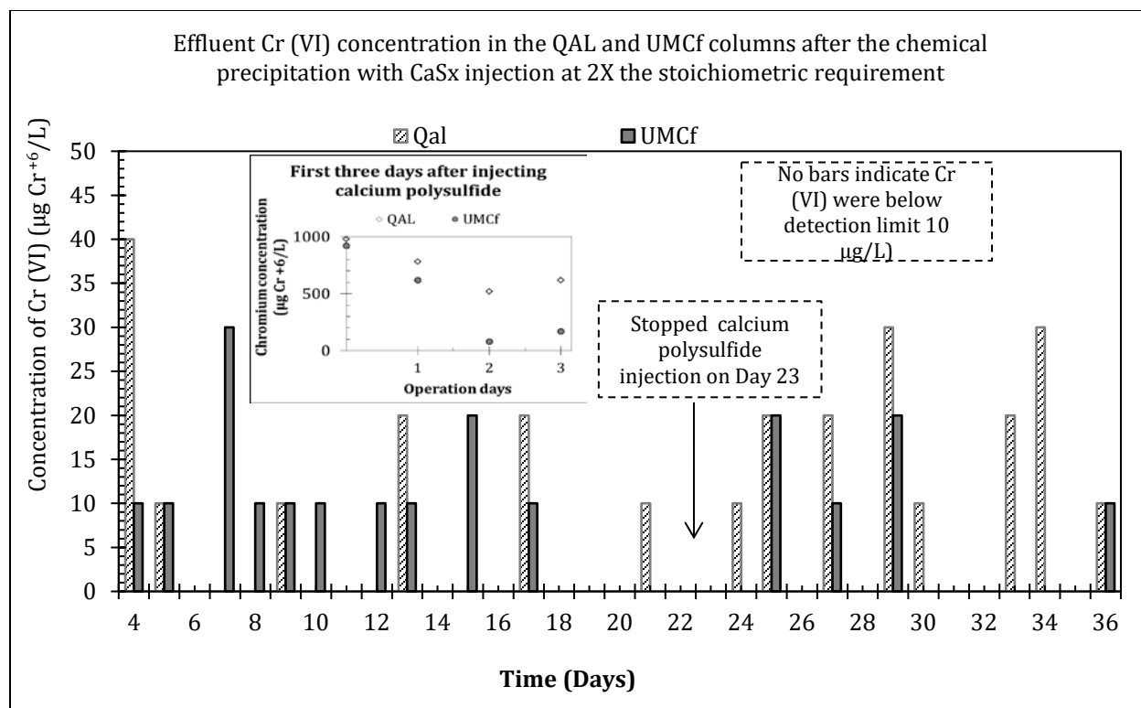
Figure D.2: Effluent Cr (VI) concentrations in the QAL and the UMCf column after chemical precipitation of chromium with calcium polysulfide. The inset in the picture shows chromium concentration in composite samples in days 1 to 3. (Calcium polysulfide was stopped on Day 23 represented by an arrow). The average influent hexavalent chromium concentration was 980 \pm 0.01 \text{ mg/L} and 960 \pm 0.5 \mu\text{g/L} in QAL and UMCf, respectively. CaSx was fed continuously in QAL column, and was injected each day in UMCf column.
