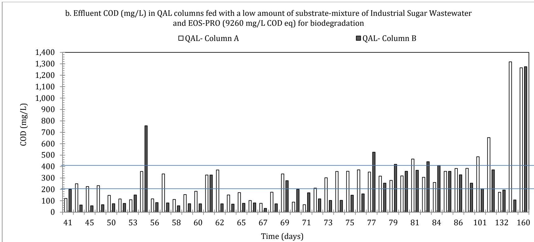
Figure 5.31: COD in the QAL columns- a high amount of substrate (mixture of Industrial Sugar Wastewater at 7% and EOS-PRO at 2% by volume) with 45880 mg/L COD eq, no substrate and EOS-PRO alone at 0.2% (4000 mg/L COD eq) and 0.4% (8000 mg/L COD eq) (a) and a low amount of substrate (mixture of Industrial Sugar Wastewater at 1.5% and EOS-PRO at 0.4%) with 9260 mg/L COD eq (b). The average influent hexavalent chromium concentration in the columns were 14261 \pm 1987 \mu\text{g/L} (a) and 12377 \pm 997 \mu\text{g/L} (b) over the operation periods. (The horizontal lines are drawn to clarify the 200 mg/L and 400 mg/L COD levels).
