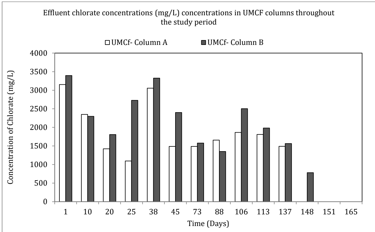
Figure 5.40: Effluent chlorate concentrations in the UMCf.
