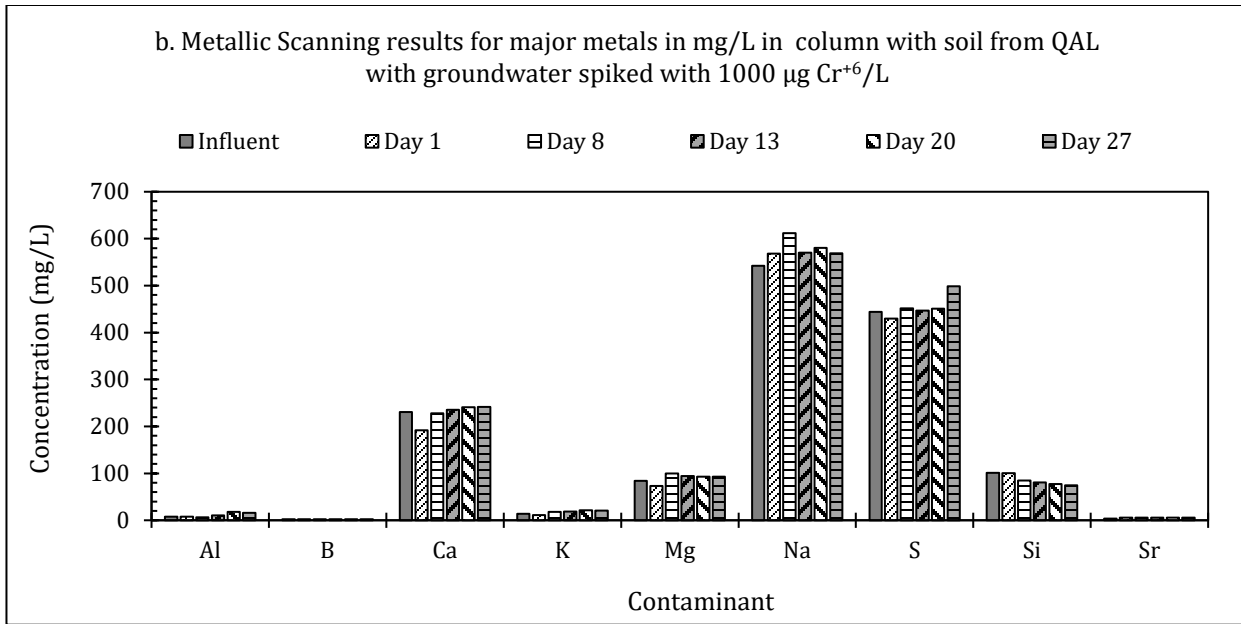
Figure 4.8: Total metal concentrations in the QAL in \mu\text{g}/\text{L} (a) \text{mg}/\text{L} (b).
