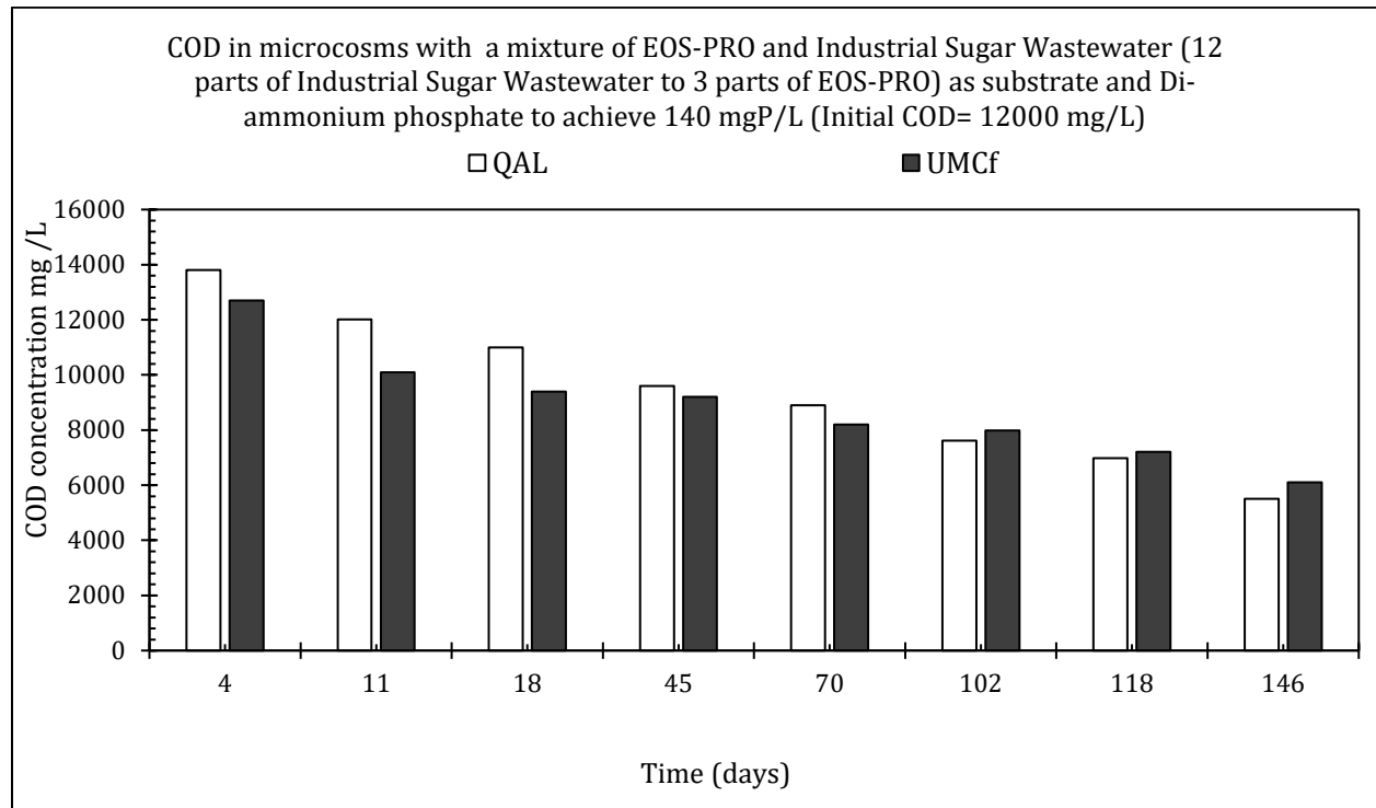
Figure 5.21: COD in QAL and UMCf microcosms with a mixture of EOS-PRO and Industrial Sugar Wastewater as substrate.
