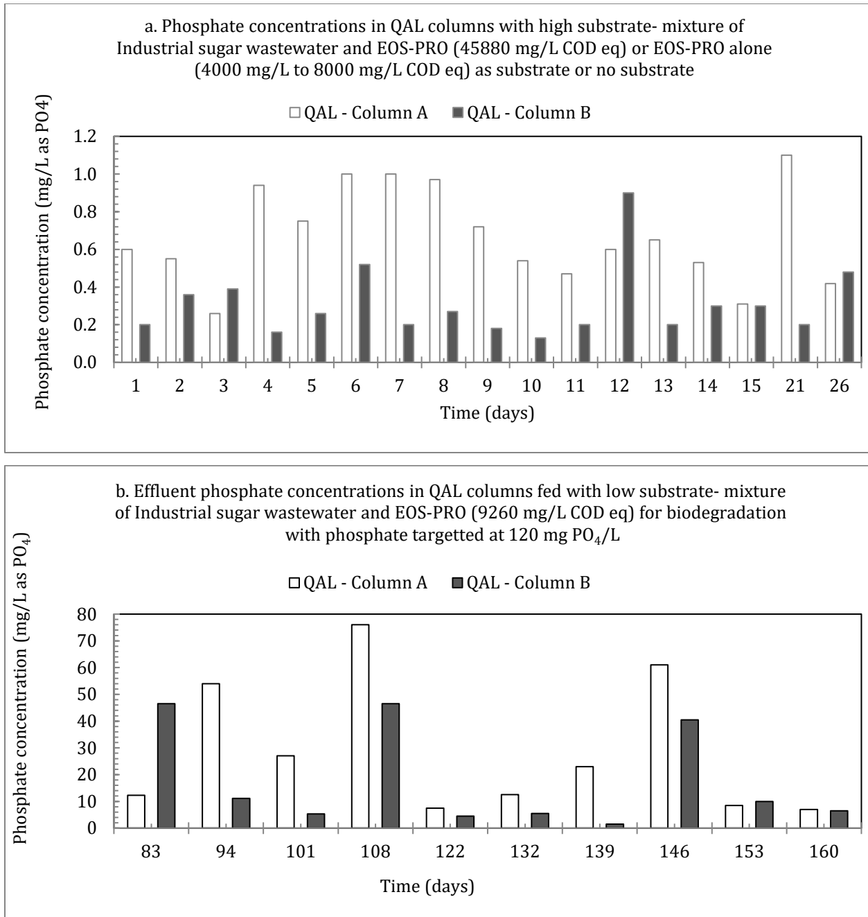
Figure 5.44: Effluent phosphate concentrations in the QAL.
