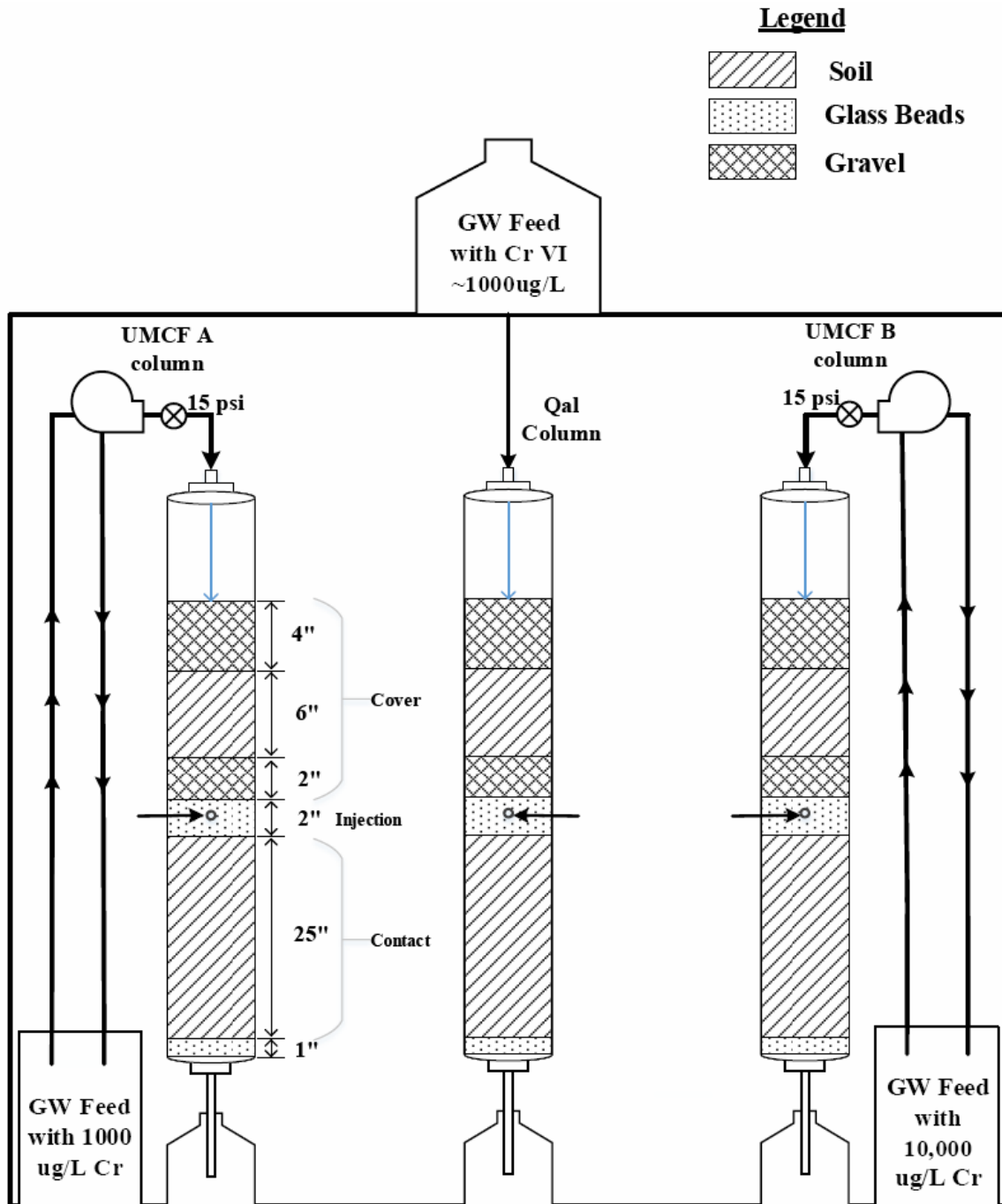
Figure 2.2: Schematic diagram of columns for chemical precipitation of chromium in columns using calcium polysulfide. The horizontal arrows at 27 inches from the bottom of the column indicate the injection port for calcium polysulfide.
