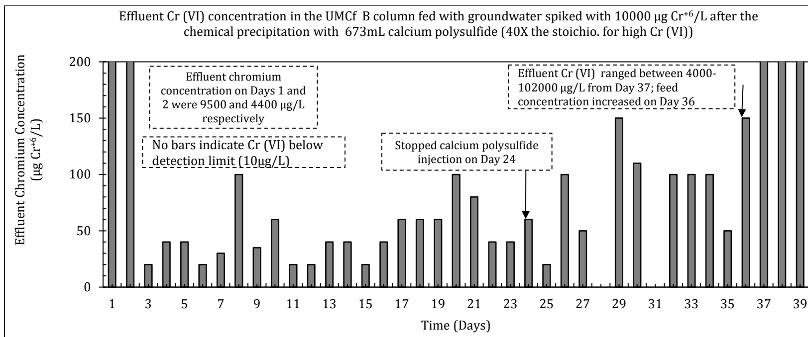
Figure 4.4: Effluent Cr (VI) concentrations in the UMCf B after chemical precipitation of chromium with calcium polysulfide. (CaSx was stopped on Day 24 represented by an arrow). The average influent Cr (VI) concentration was 9639 \pm 465 \mu\text{g/L} and percent removal of 93 \pm 22\% in the column during the injection period.
