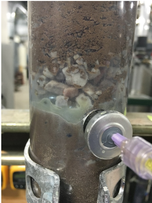
Figure F.9: Injection port on QAL column Day 5 shows the white scale formation at the injection port
