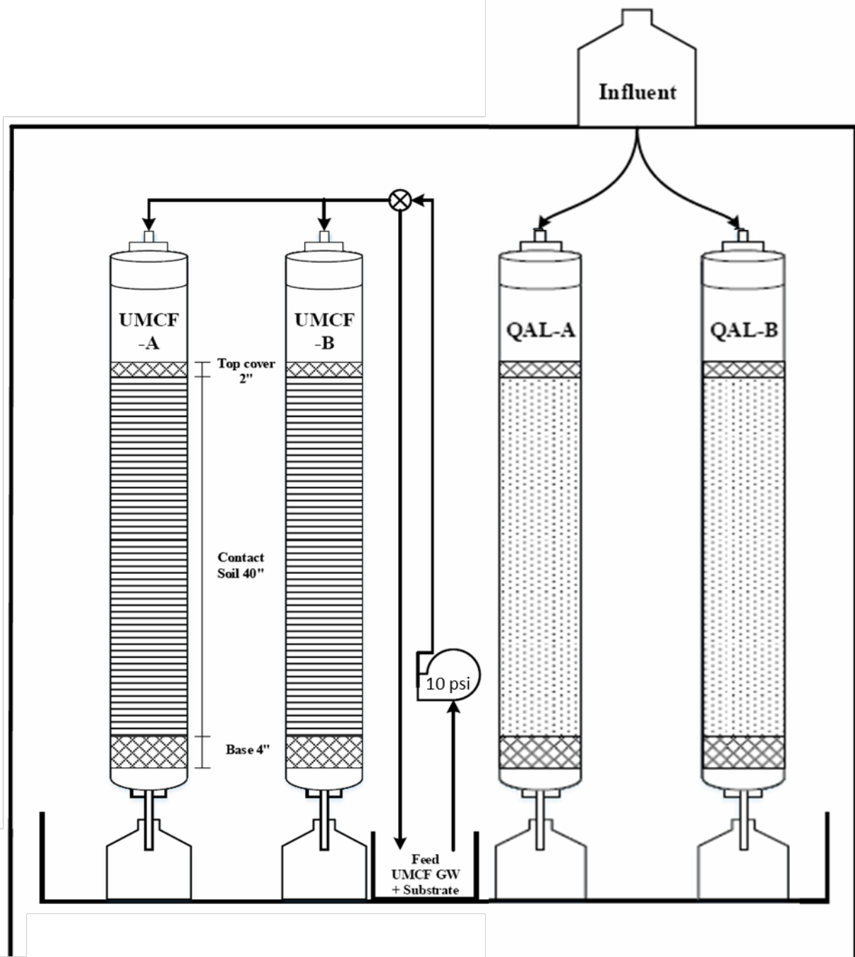
Figure 2.4: Schematic diagram of columns used for biological treatment of the UMCF and QAL contaminated groundwater (Day 1 to Day 28).
