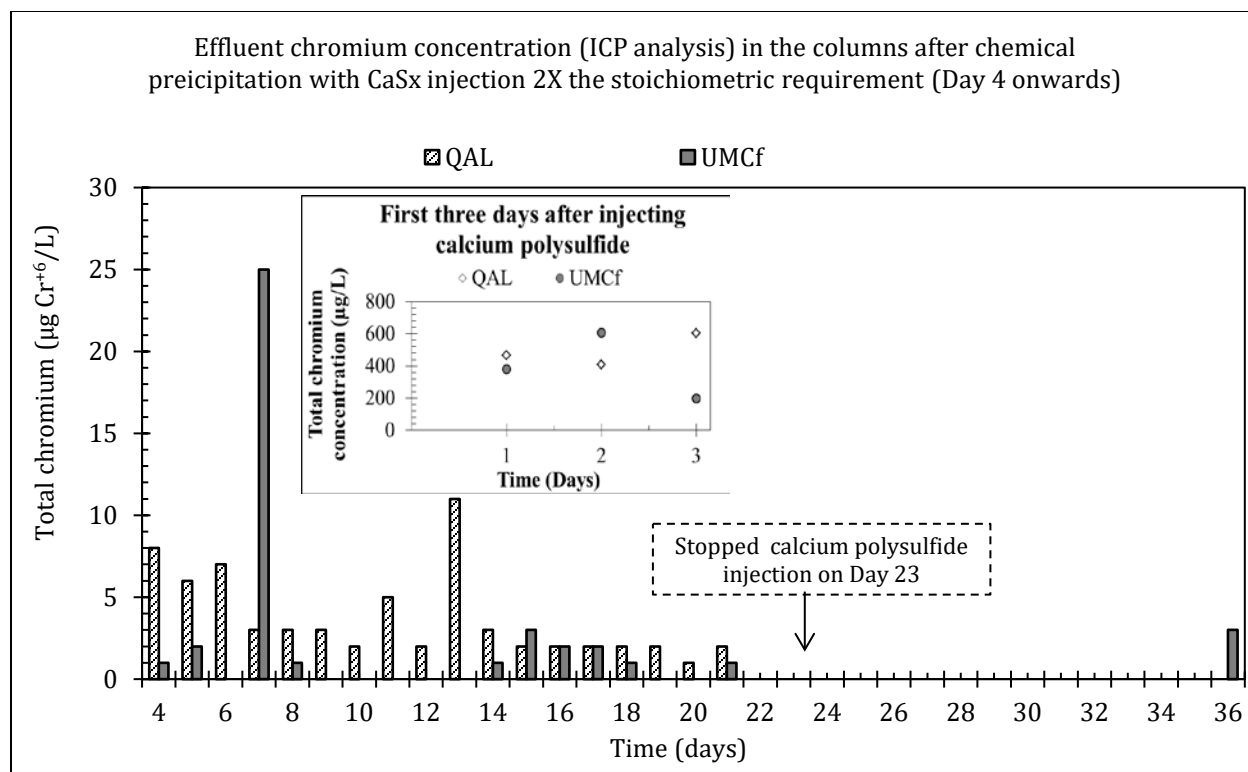
Figure D.3: Effluent dissolved chromium concentrations in the QAL and the UMCf column after chemical precipitation of chromium with calcium polysulfide from Day 4. The indent in the picture shows chromium concentration in composite samples in days 1 to 3. (Calcium polysulfide was stopped on Day 23 represented by the vertical arrow). Note that in columns, most of the precipitate was trapped by the soil media resulting in lower value of total chromium after sample filtration.
