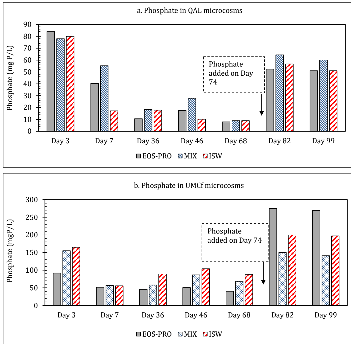
Figure 5.14: Phosphate concentration in the QAL (a) and UMCf (b) microcosms.
