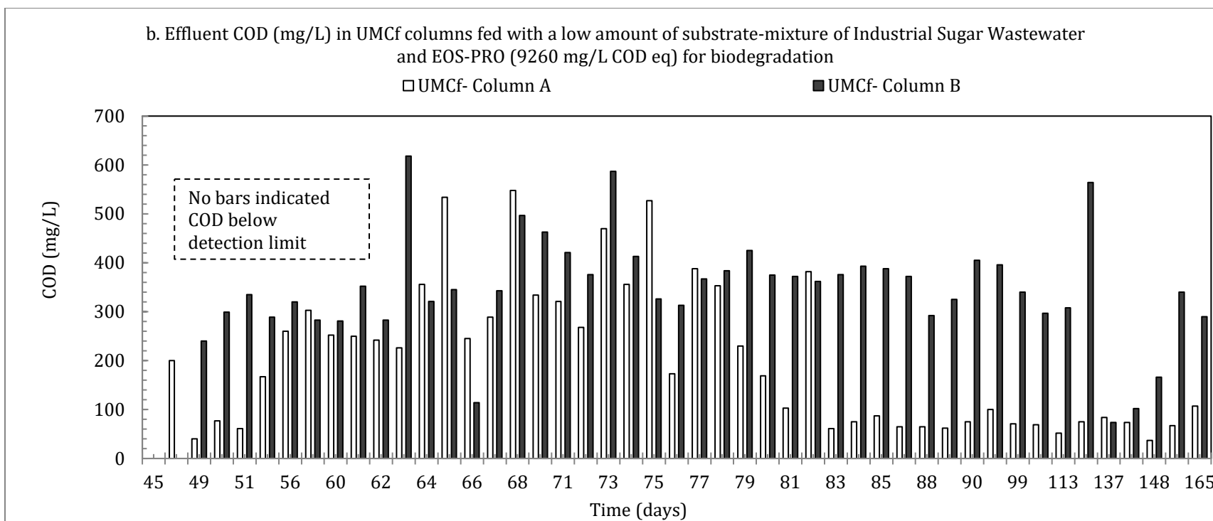
Figure 5.32: Effluent COD in the UMCf columns fed with a high amount of substrate (mixture of Industrial Sugar Wastewater at 7% and EOS-PRO at 2% by volume) with 45880 mg/L COD eq, no substrate and EOS-PRO alone at 0.2% (4000 mg/L COD eq) and 0.4% (8000 mg/L COD eq) (a) and a low amount of substrate (mixture of Industrial Sugar Wastewater at 1.5% and EOS-PRO at 0.4%) with 9260 mg/L COD eq (b). The average influent hexavalent chromium concentration was 17385 \pm 1829 \mu\text{g/L} (a) and 15360 \pm 1325 \mu\text{g/L} (b) over the operation periods.
