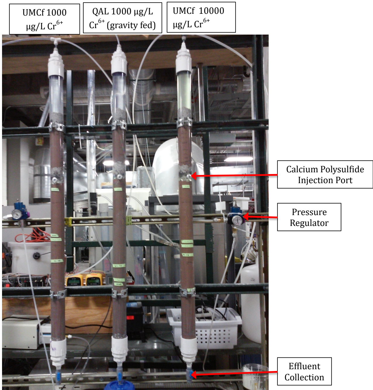
Figure F.11: Set-up of the Final columns for Cr Treatment with CaSX
