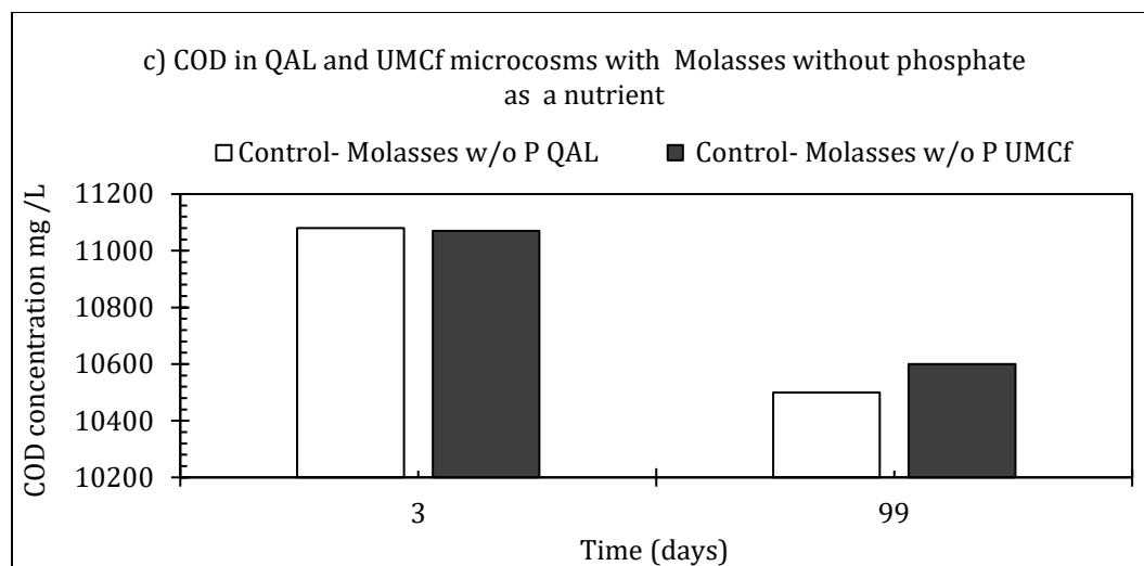
Figure 5.3: COD in QAL and UMCf control microcosm: blank (a), Industrial Sugar Wastewater without phosphate (b), and Molasses without phosphate (c).
