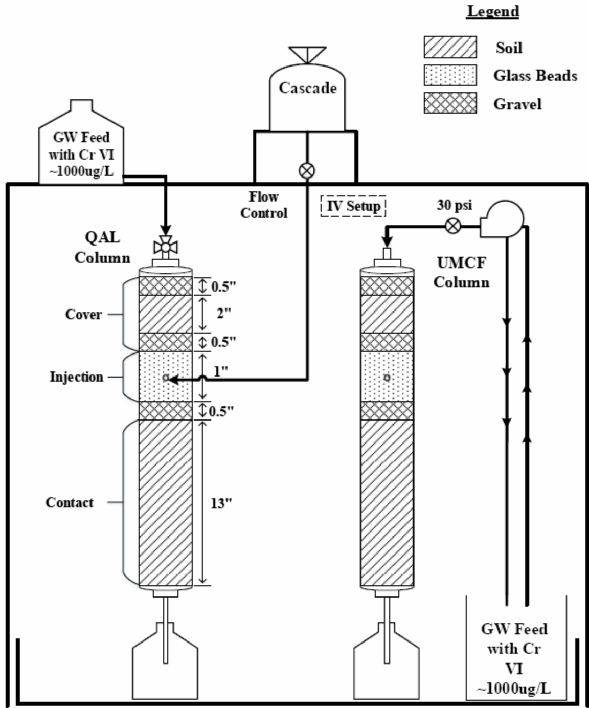
Figure D.1: Schematic diagram of the preliminary columns to remove chromium with CaSx
