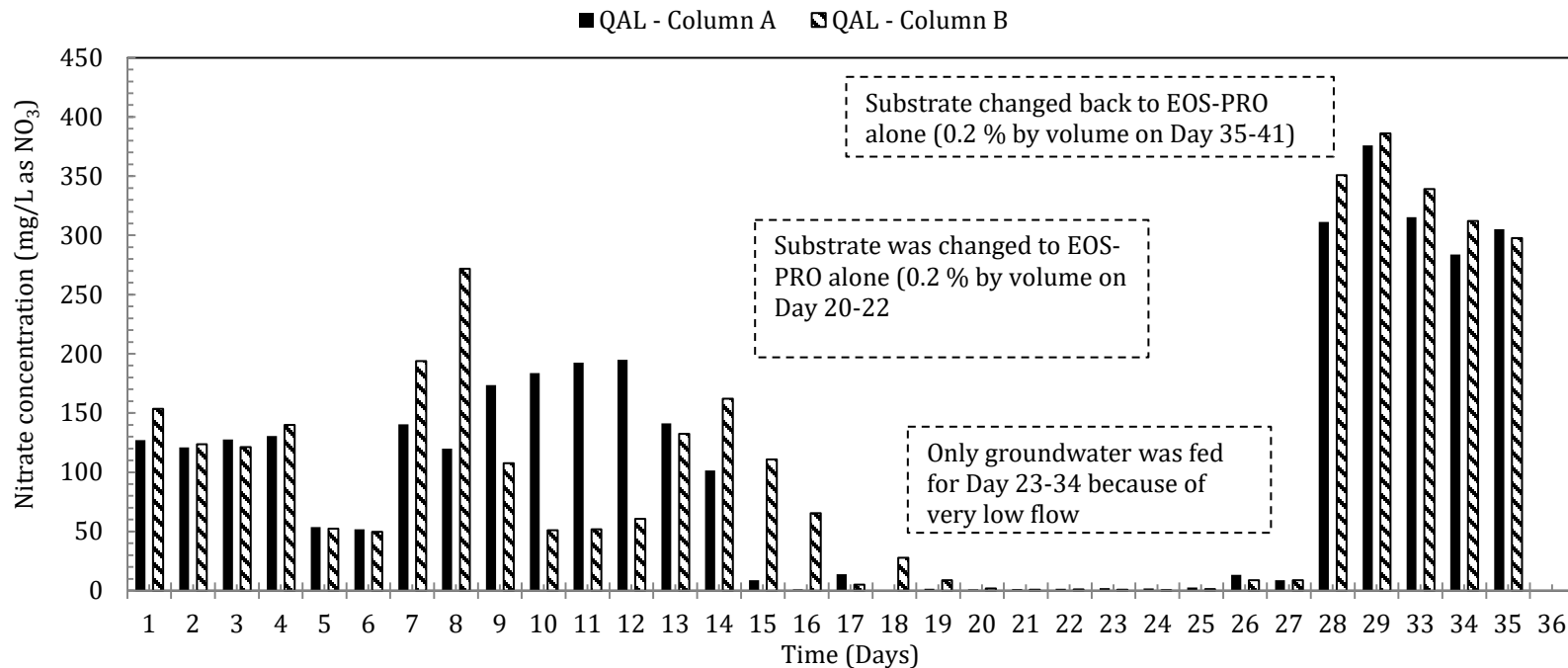
a. Effluent nitrate concentrations (mg/L as NO 3 ) concentrations in QAL columns fed with a high amount of substrate - mixture of Industrial Sugar Wastewater and EOS-PRO (45880 mg/L COD eq ) or EOS-PRO alone (4000 mg/L to 8000 mg/L COD eq) as substrate or n
