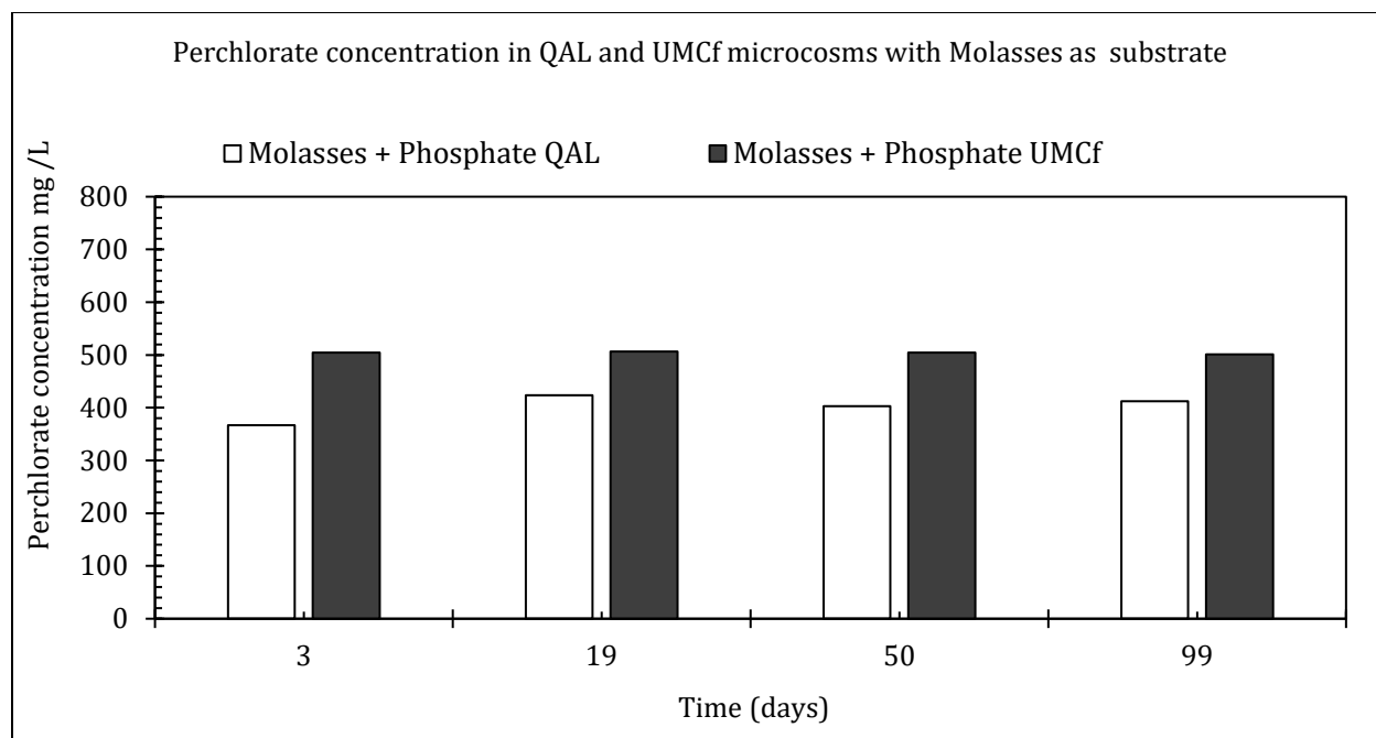
Figure 5.13: Perchlorate concentration in Molasses in QAL and UMCf microcosms.
