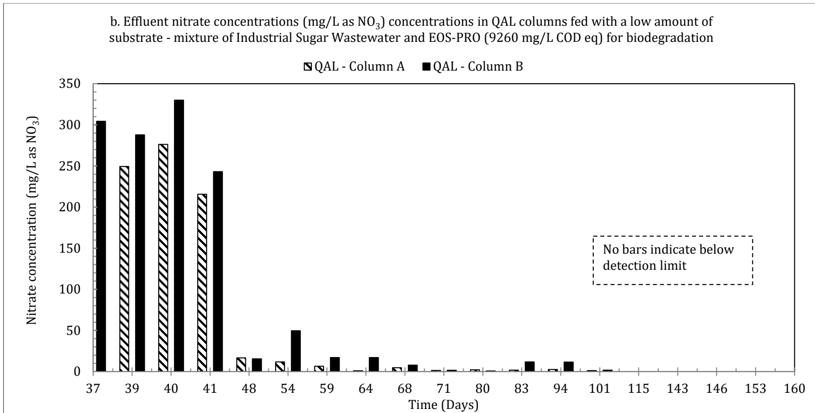
Figure 5.37: Effluent nitrate concentrations in the QAL.
