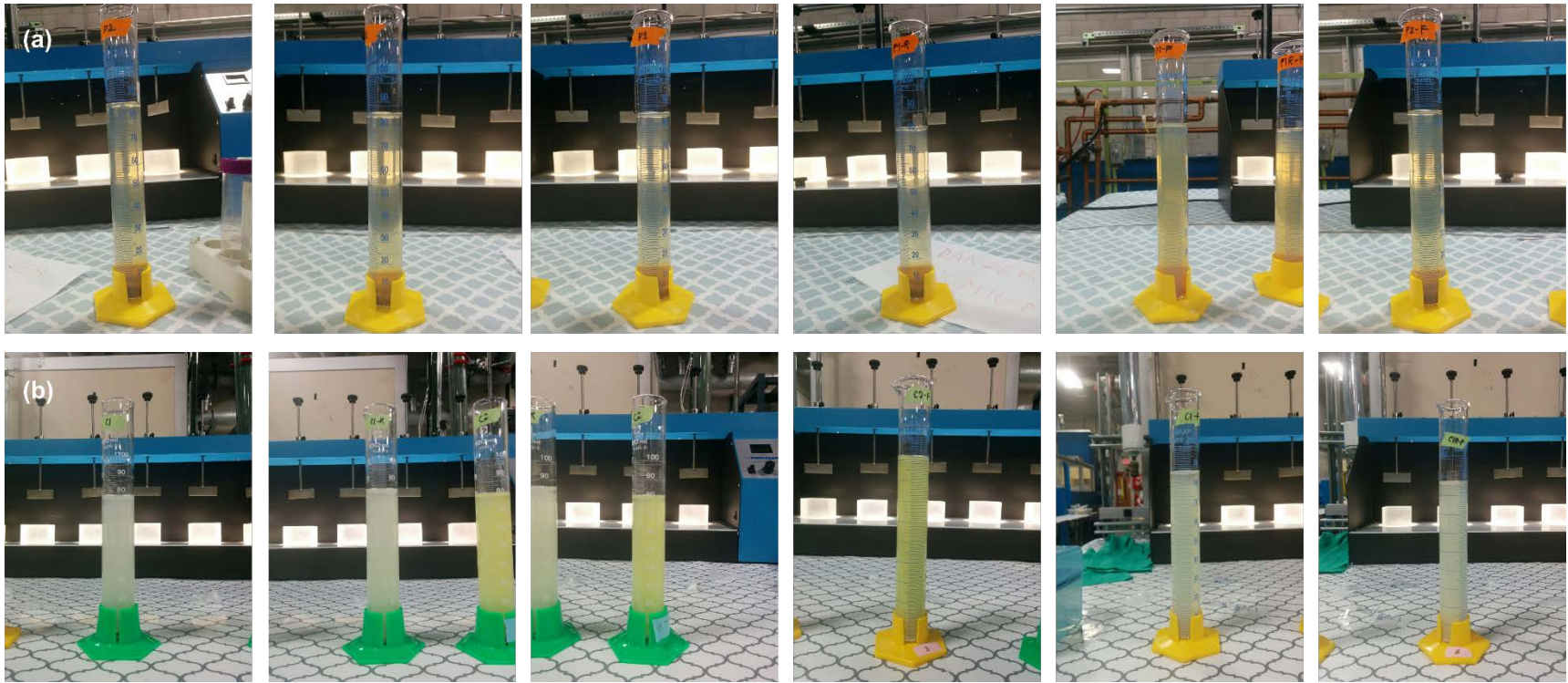
Figure F.2: High-range concentration settling: (a) groundwater with ferrous sulfate and (b) with calcium polysulfide.
