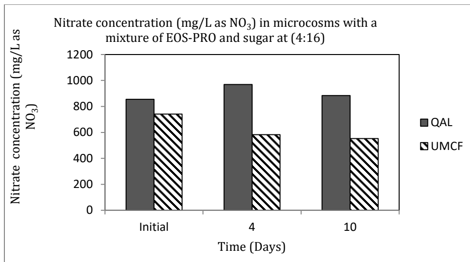
Figure 5.30: Nitrate in QAL and UMCf microcosms with a mixture of EOS-PRO and sugar as substrate.
