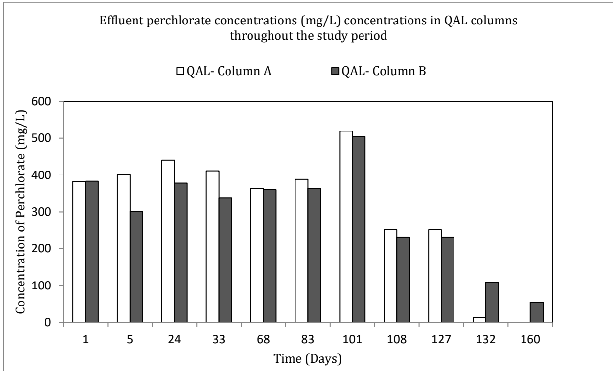
Figure 5.41: Effluent perchlorate concentrations in the QAL.
