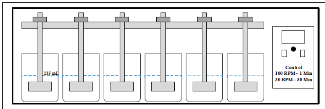
Figure 2.1 Experimental setup used in the batch tests for chromium precipitation with \text{CaSx} and \text{FeSO}_4 .
