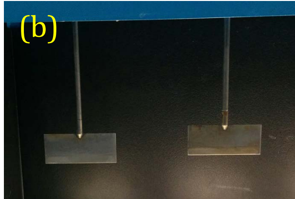
Figure F.6: Stirrers after operating batch precipitation test with groundwater from 25-30 ft containing high-range chromium concentration: (a) ferrous sulfate or (b) with calcium polysulfide showing that no inorganic scales were formed on the stirrer.
