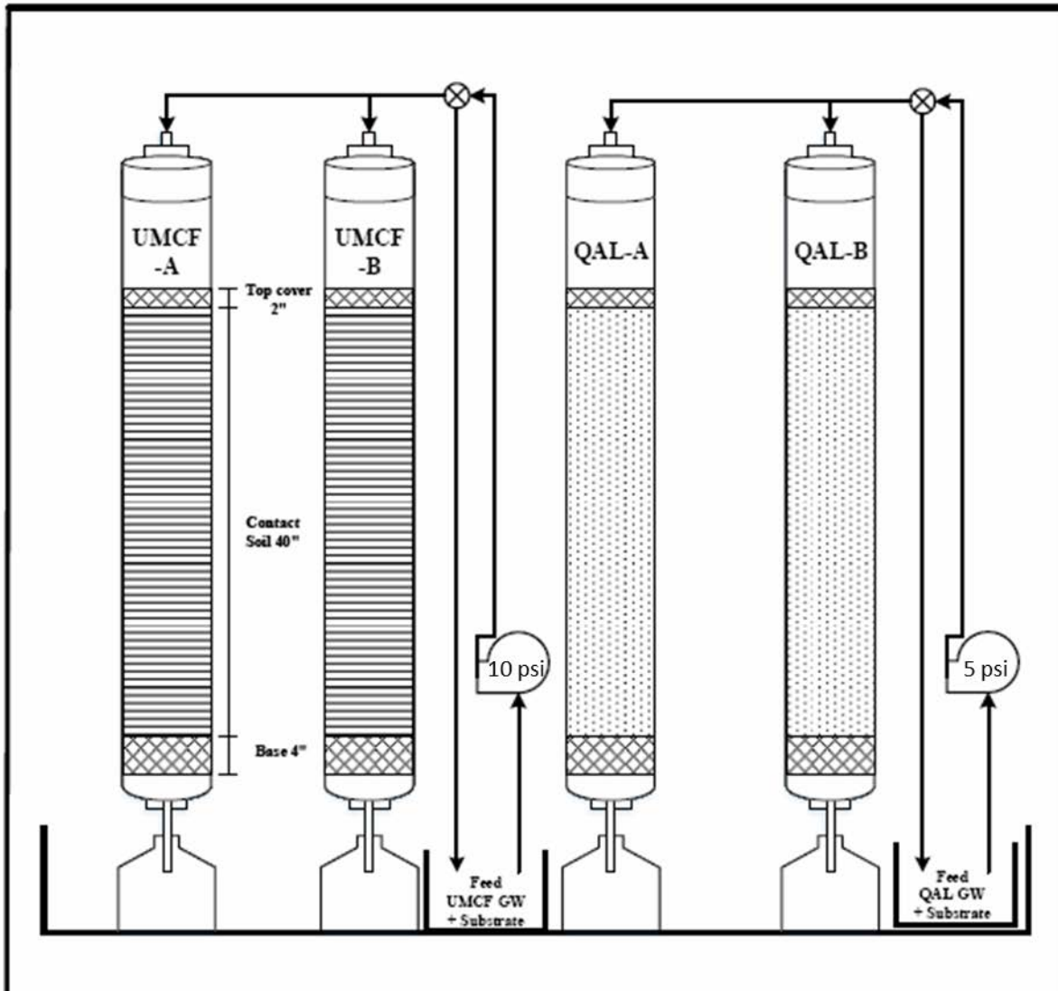
Figure 2.5: Schematic diagram of columns used for biological treatment of the QAL and UMCF groundwater after Day 28. The QAL columns were pressurized at 5 psi and UMCF was 10 psi. The QAL columns before Day 28 were gravity fed.
