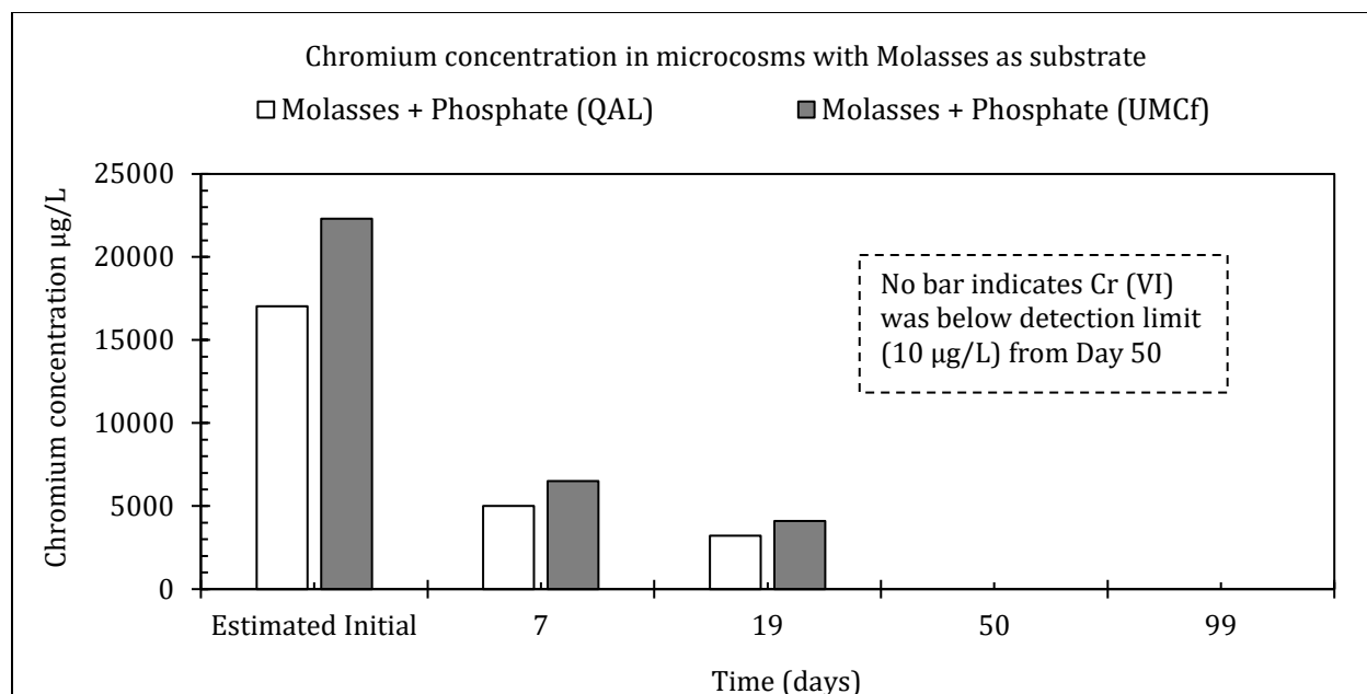
Figure 5.5: Cr (VI) in microcosms with Molasses as substrate with phosphate.
