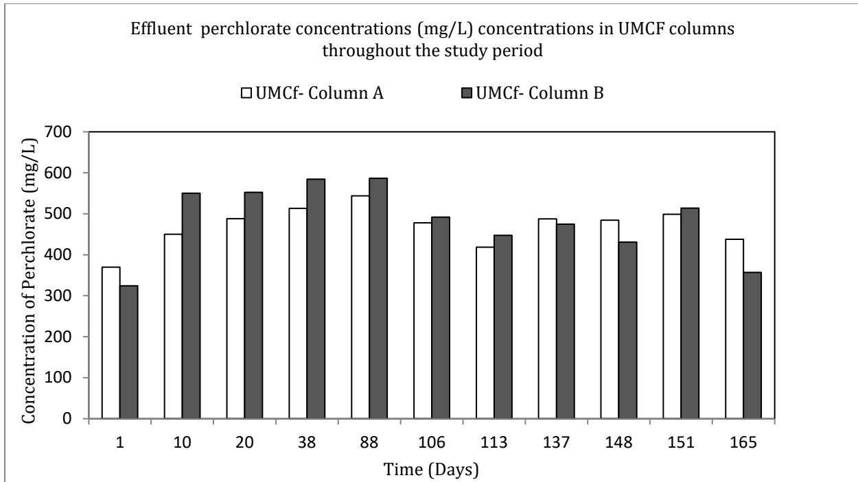
Figure 5.42: Effluent perchlorate concentrations in the UMCf.
