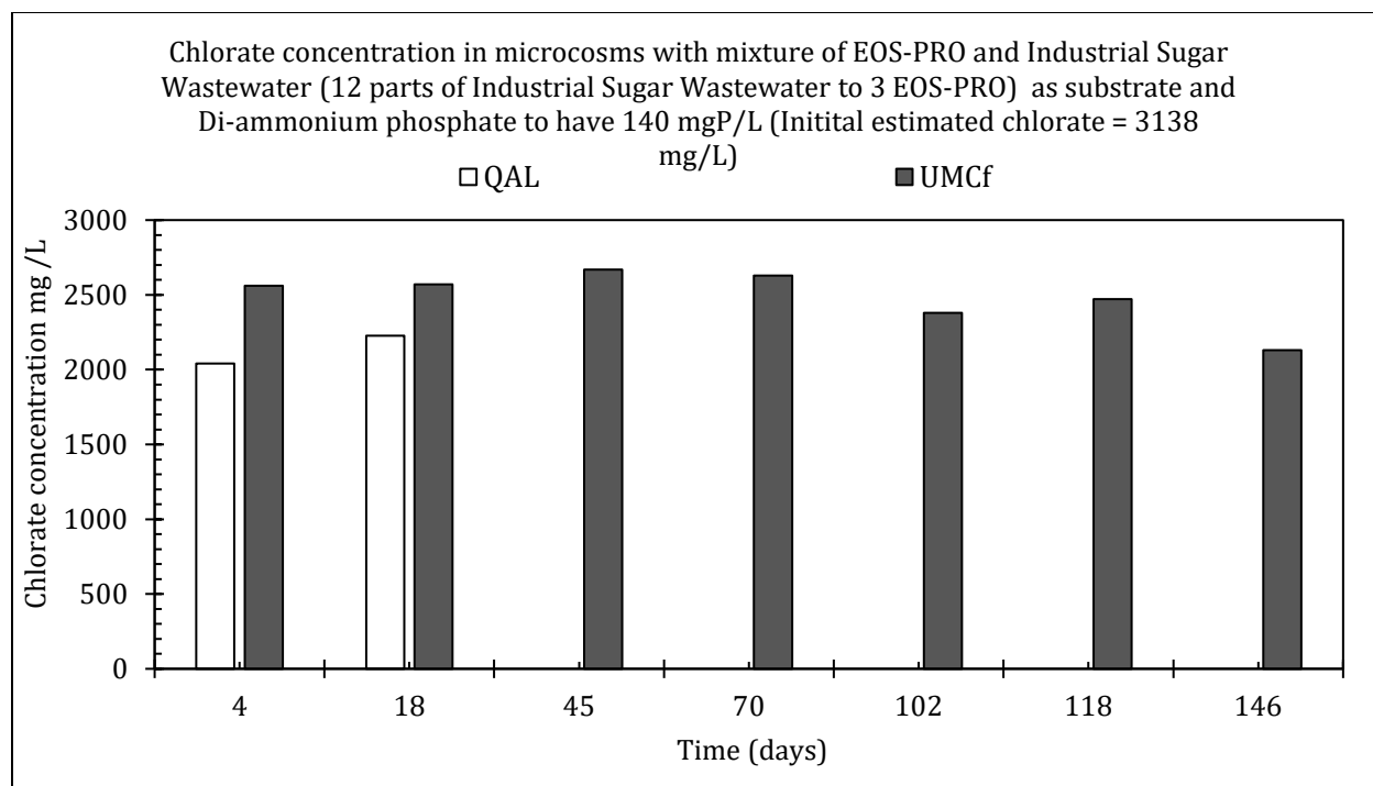
Figure 5.23: Chlorate concentration in QAL and UMCf microcosms with a mixture of EOS-PRO and Industrial Sugar Wastewater as substrate.
