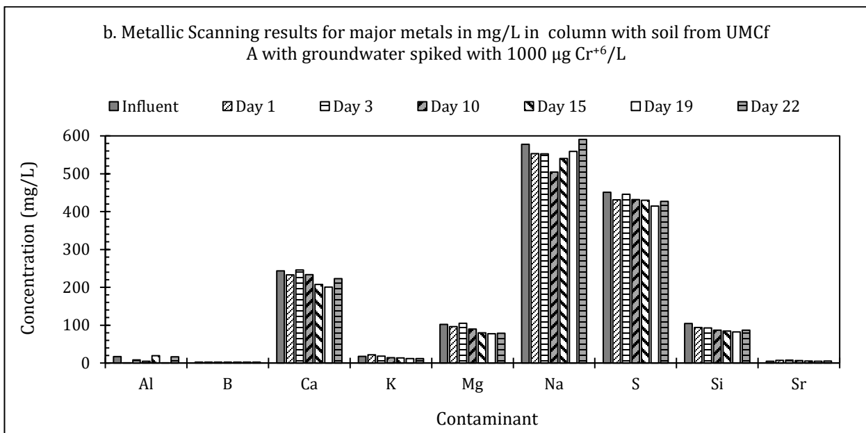
Figure 4.9: Total metal concentrations in the UMCf A in \mu\text{g/L} (a) \text{mg/L} (b).
