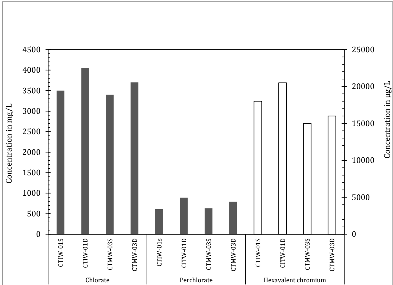
Figure 3.7: Groundwater from well CTIW 01D, CTIW 01S, CTMW 03, and CTMW 03D analysis obtained from Tetrtech
