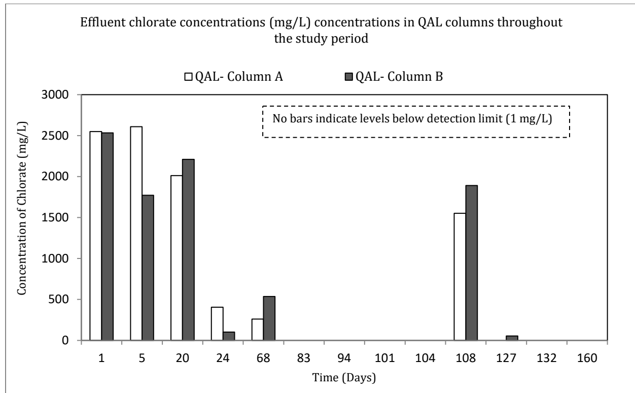
Figure 5.39: Effluent chlorate concentrations in the QAL.
