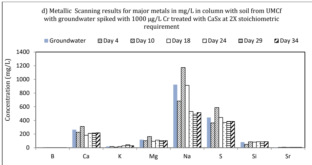
Figure D.4: Scanning of trace and major results in effluent in the QAL (a and b) and the UMCf (c and d) columns at different days.
