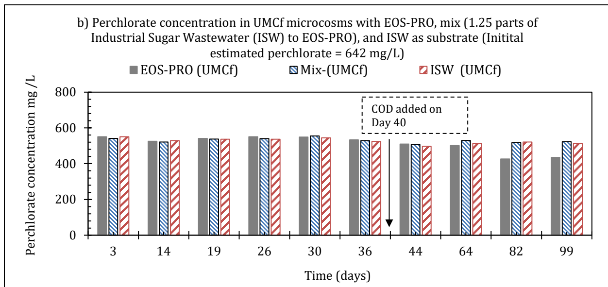
Figure 5.12: Perchlorate concentration in QAL (a), and UMCf (b) microcosms.
