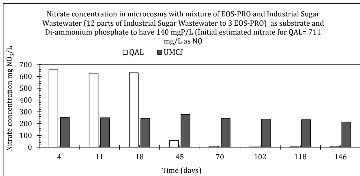
Figure 5.22: Nitrate concentration in QAL and UMCf microcosms with a mixture of EOS-PRO and Industrial Sugar Wastewater as substrate.
