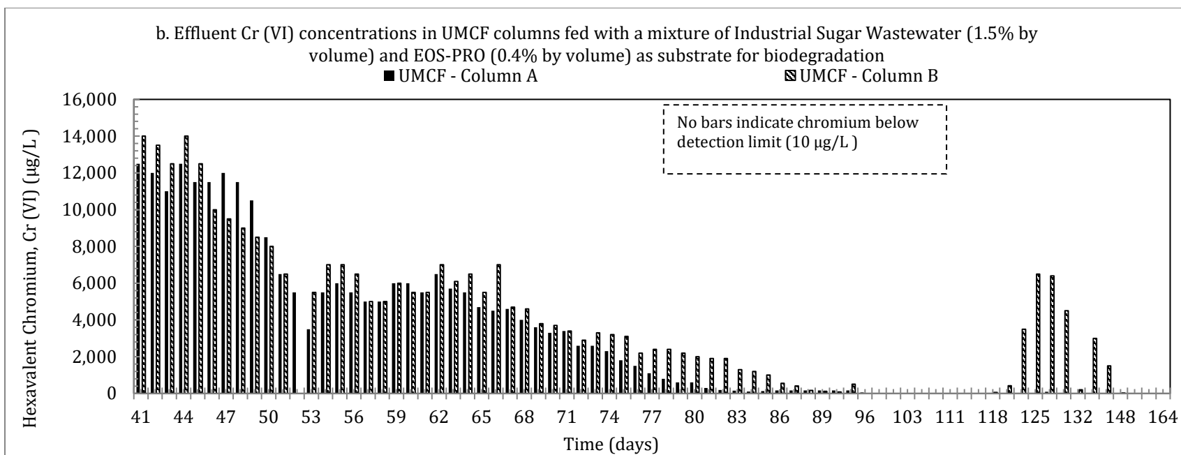
Figure 5.34: Effluent Cr (VI) concentrations in the UMCf columns fed with: a high amount of substrate (mixture of Industrial Sugar Wastewater at 7% and EOS-PRO at 2% by volume) with 45880 mg/L COD eq, no substrate and EOS-PRO alone at 0.2% (4000 mg/L COD eq) and 0.4% (8000 mg/L COD eq) (a) and a low amount of substrate (mixture of Industrial Sugar Wastewater at 1.5% and EOS-PRO at 0.4%) with 9260 mg/L COD eq (b). The average influent hexavalent chromium concentration was 17385 \pm 1829 \mu\text{g/L} (a) and 15360 \pm 1325 \mu\text{g/L} (b) over the operation periods.
