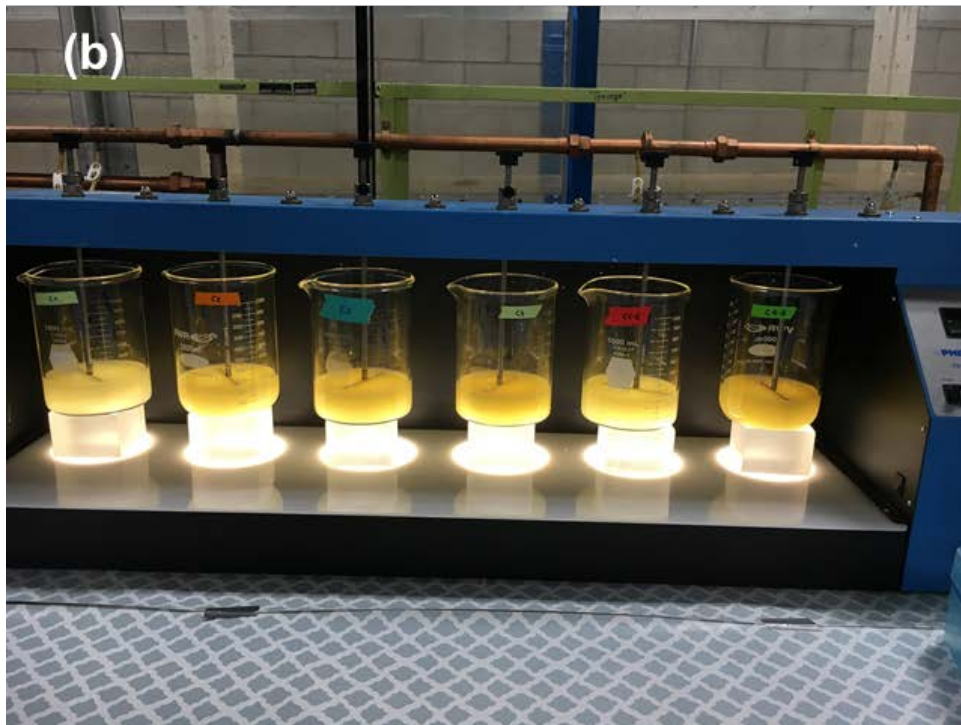
Figure F.1: High-range concentration batch experimental set-up: (a) groundwater with ferrous sulfate and (b) with calcium polysulfide.
