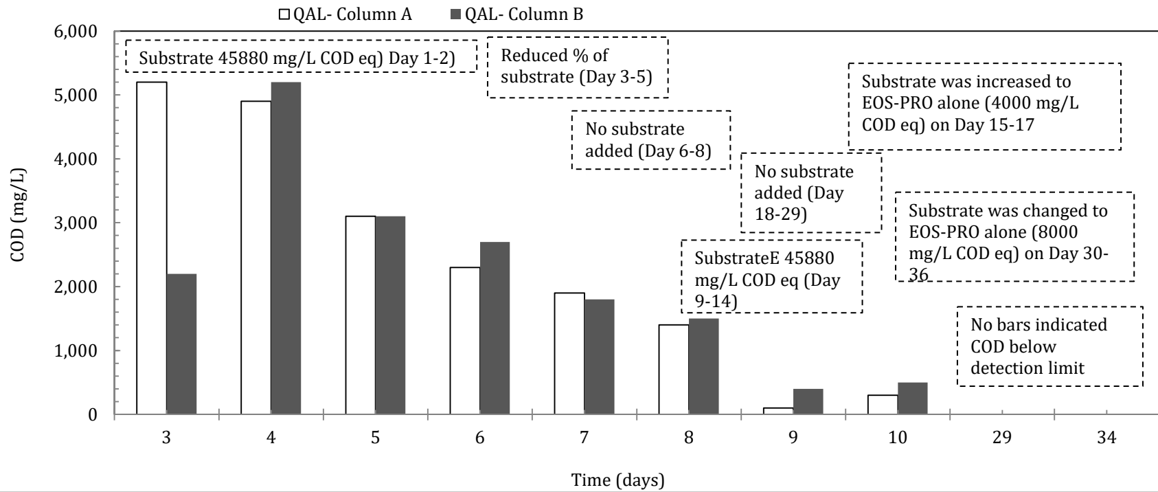
a. Effluent COD (mg/L) concentrations in QAL columns fed with high amount of substrate - mixture of Industrial Sugar Wastewater and EOS-PRO (45880 mg/L COD eq) or EOS-PRO alone (4000 mg/L to 8000 mg/L COD eq) as substrate or no substrate
