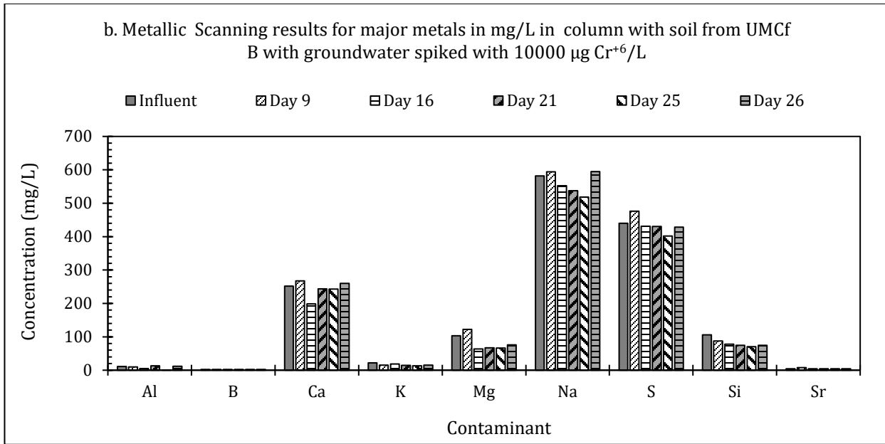
Figure 4.10: Total metal concentrations in the UMCf B in \mu\text{g}/\text{L} (a) \text{mg}/\text{L} (b).
