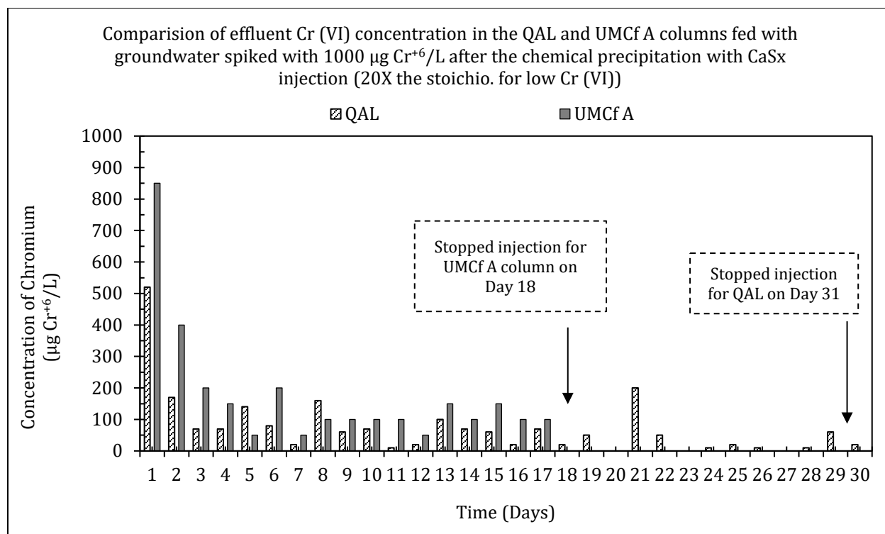
Figure 4.3: Comparison of effluent Cr (VI) concentrations in grab samples in the the QAL and UMCf A column during the injection of calcium polysulfide. (The days when the calcium polysulfide stopped are represented by arrows). The average influent hexavalent chromium concentration was 1163 \pm 121 µg/L in QAL and 876 \pm 171 µg/L in UMCf.
