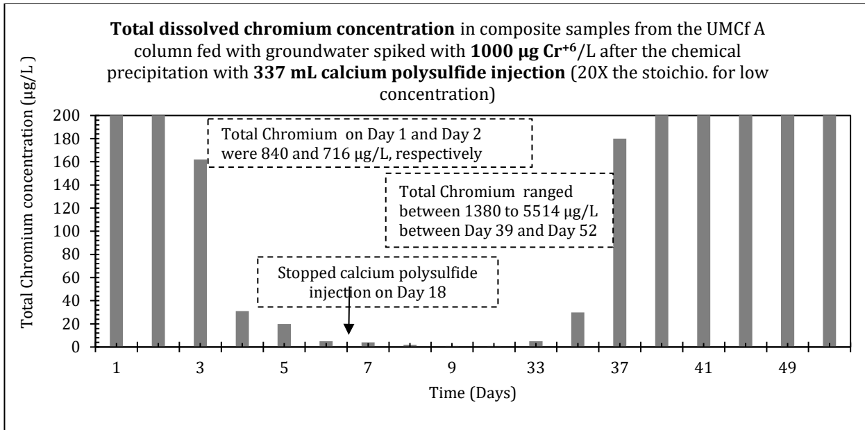
Figure 4.6: Total dissolved chromium concentrations measured in settled, but unfiltered composite samples in the UMCf A column throughout the study period. The vertical arrow indicates the day when the calcium polysulfide injection was stopped for each column.
