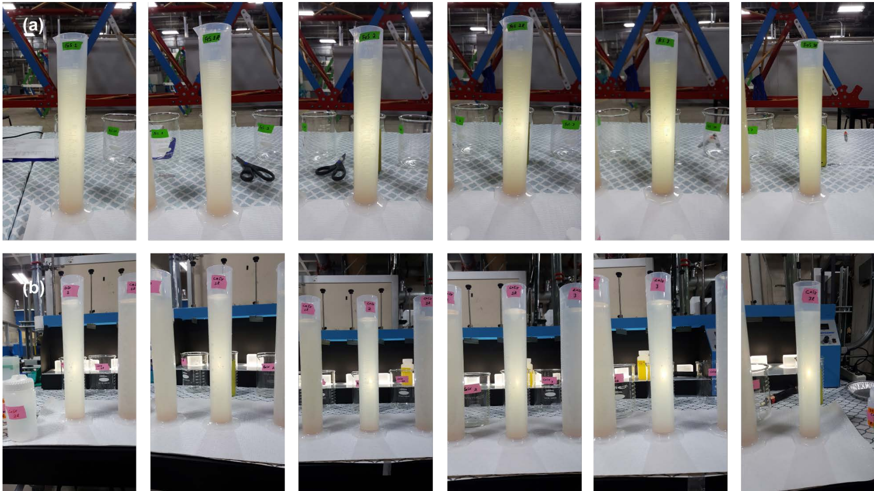
Figure F.4: Low-range concentration settling for QAL groundwater (25-30 feet bgs): (a) groundwater with ferrous sulfate and (b) with calcium polysulfide. Each set shows the sludge of individual tests.
