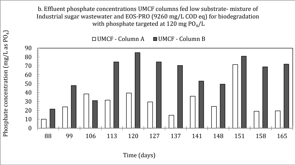
Figure 5.45: Effluent phosphate concentrations in the UCMf.
