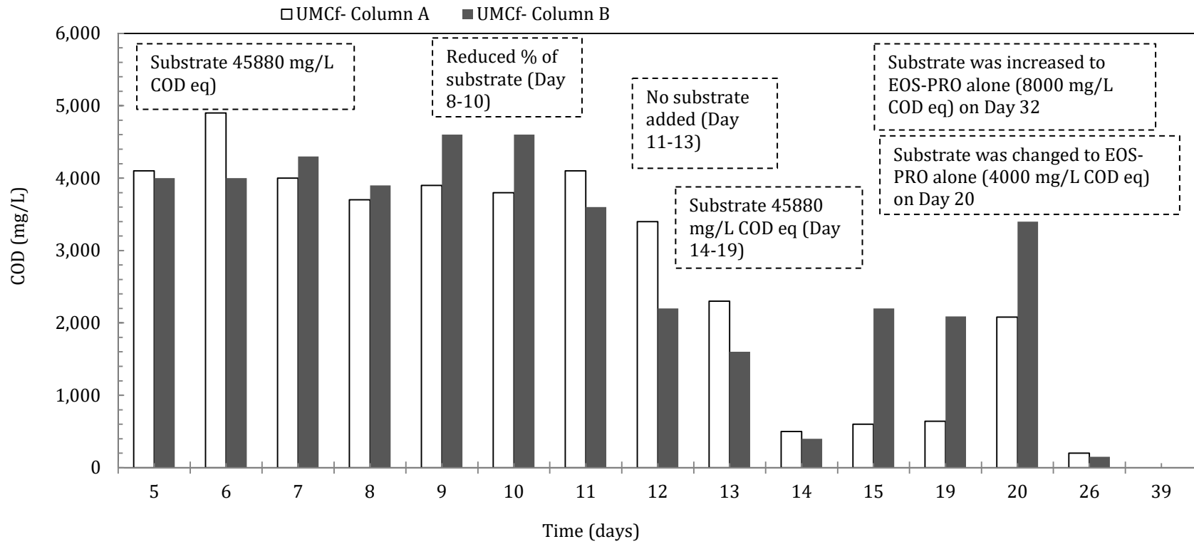
a. Effluent COD (mg/L) concentrations in UMCf columns fed with high amount of substrate - mixture of Industrial Sugar Wastewater and EOS-PRO (45880 mg/L COD eq) or EOS-PRO alone (4000 mg/L to 8000 mg/L COD eq) as substrate or no substrate
