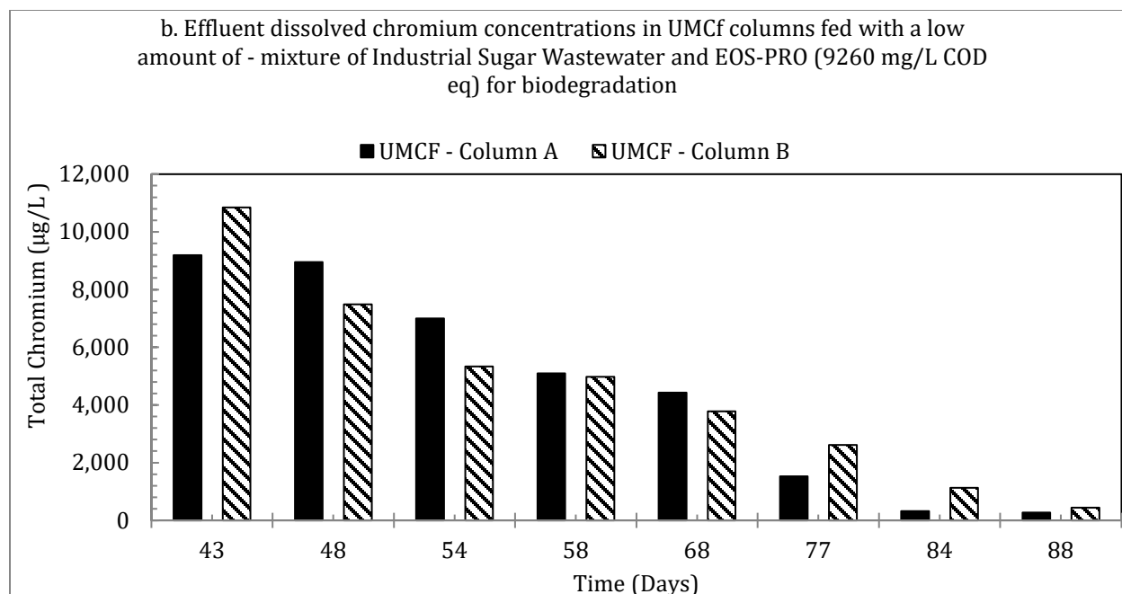
Figure 5.36: Dissolved chromium concentrations in the UMCf columns fed with- a high amount of substrate (mixture of Industrial Sugar Wastewater at 7% and EOS-PRO at 2%), no substrate and EOS-PRO alone at 0.2% and 0.4% (a) and a low amount of substrate (mixture of Industrial Sugar Wastewater at 1.5% and EOS-PRO at 0.4%) (b).
