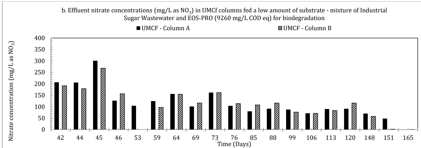
Figure 5.38: Effluent nitrate concentrations in the UMCf.
