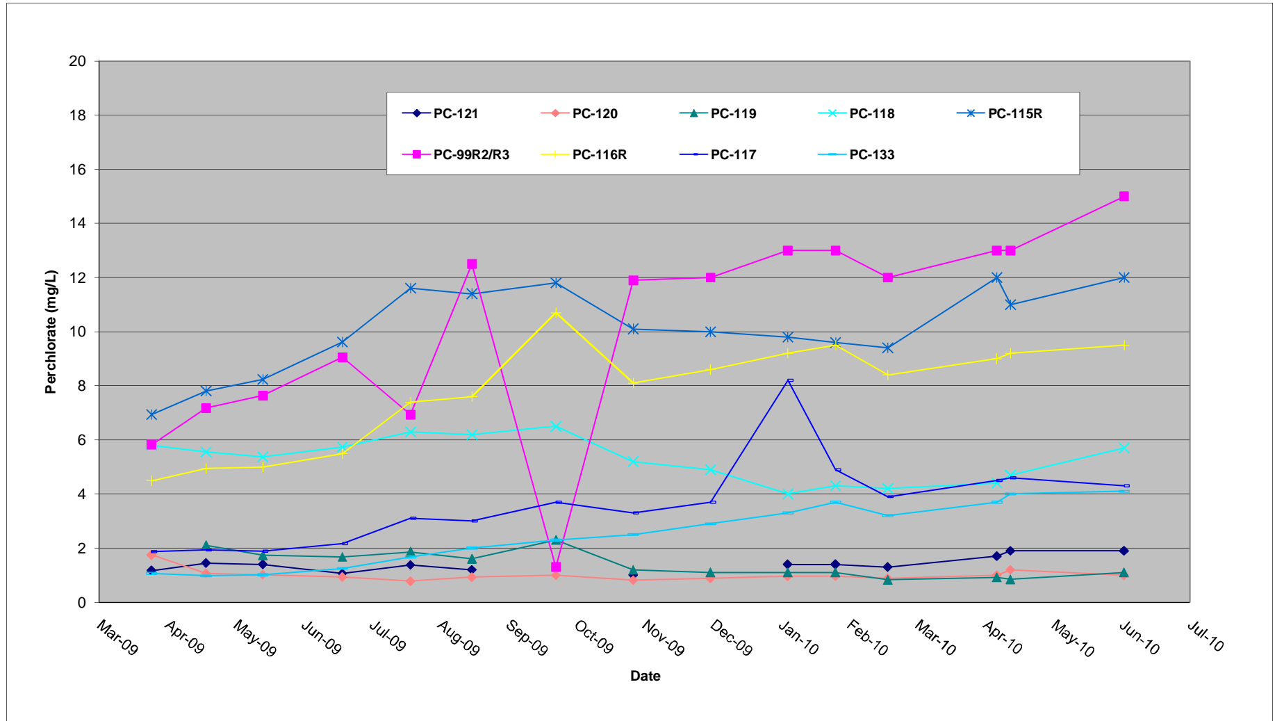
FIGURE 27A SEEP WELL FIELD PERCHLORATE CONCENTRATION TREND GRAPH APRIL 2009 TO JUNE 2010
