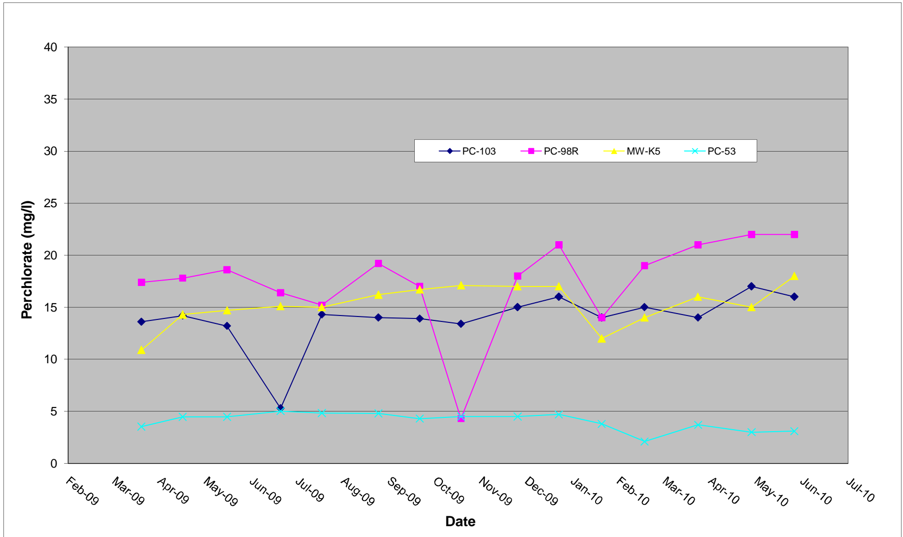
FIGURE 22A CITY OF HENDERSON WRF WELL LINE PERCHLORATE CONCENTRATION TREND GRAPH APRIL 2009 TO JUNE 2010
