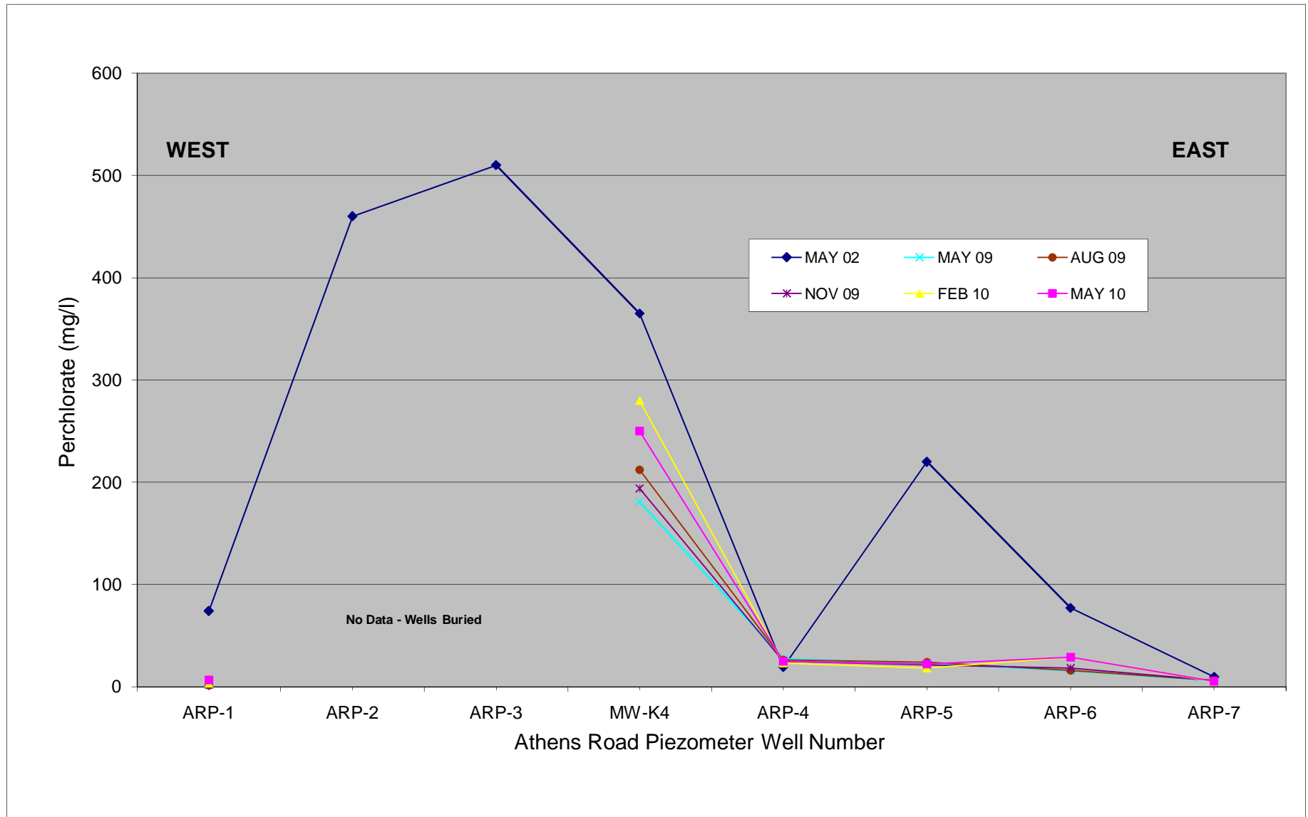
FIGURE 20 ATHENS ROAD PIEZOMETER WELLS PERCHLORATE CONCENTRATION TREND GRAPH
