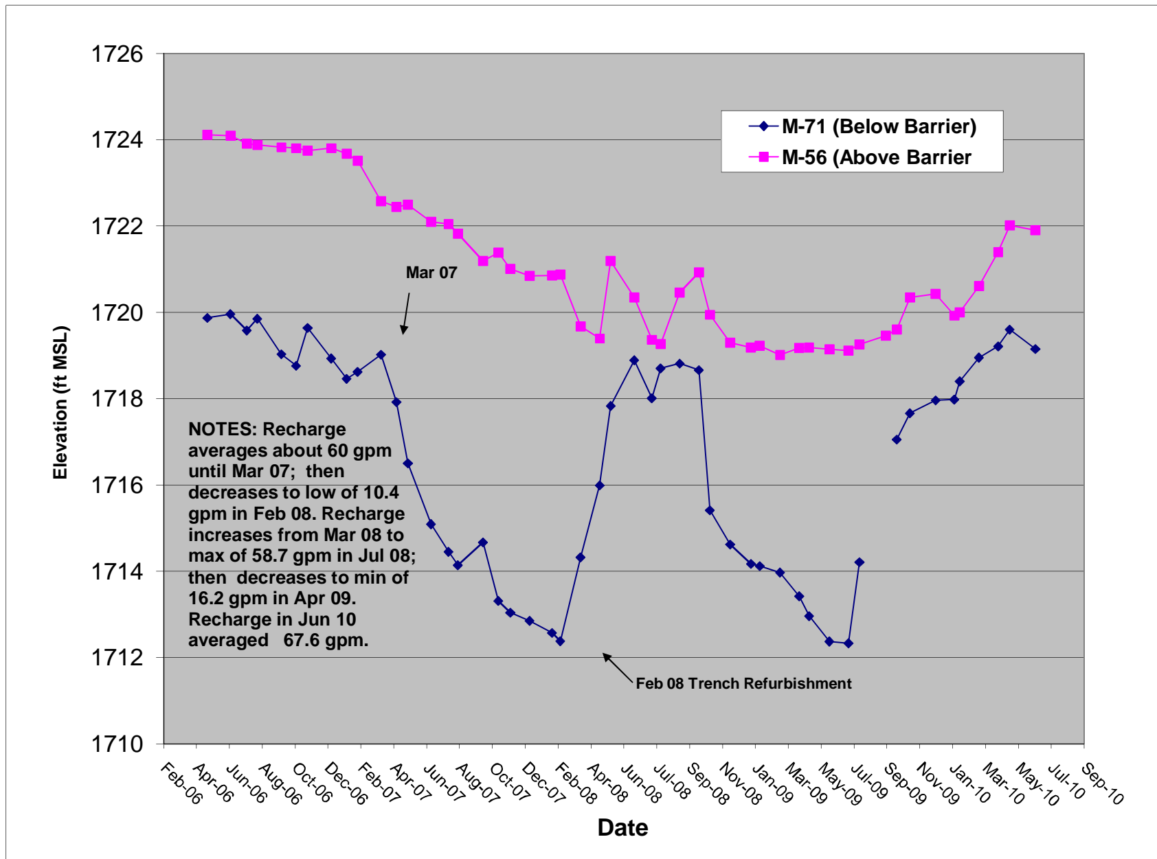
FIGURE 2 HYDROGRAPH PAIRS ACROSS THE BARRIER WALL
