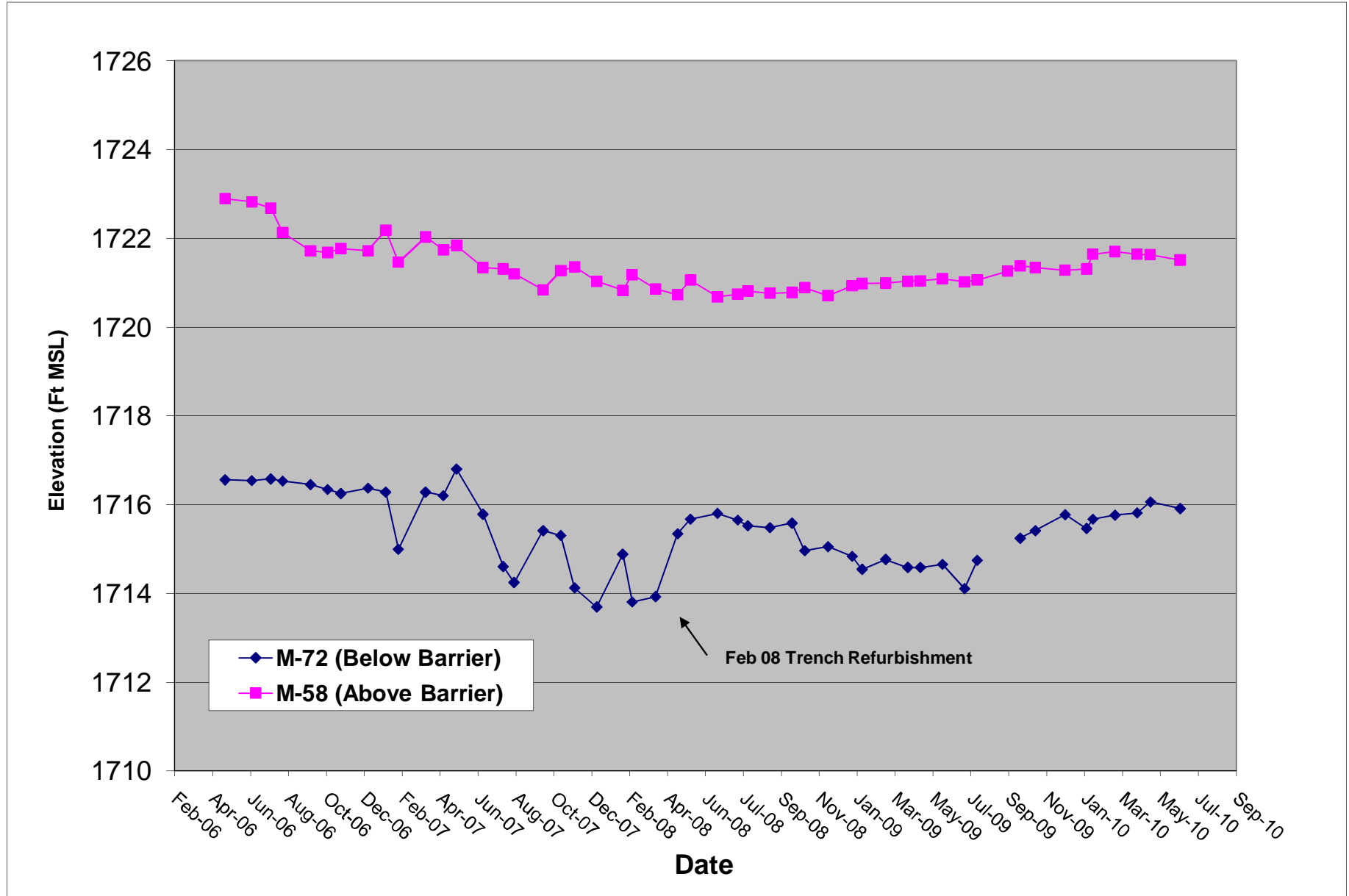
FIGURE 2 HYDROGRPAH PAIRS ACROSS THE BARRIER WALL
