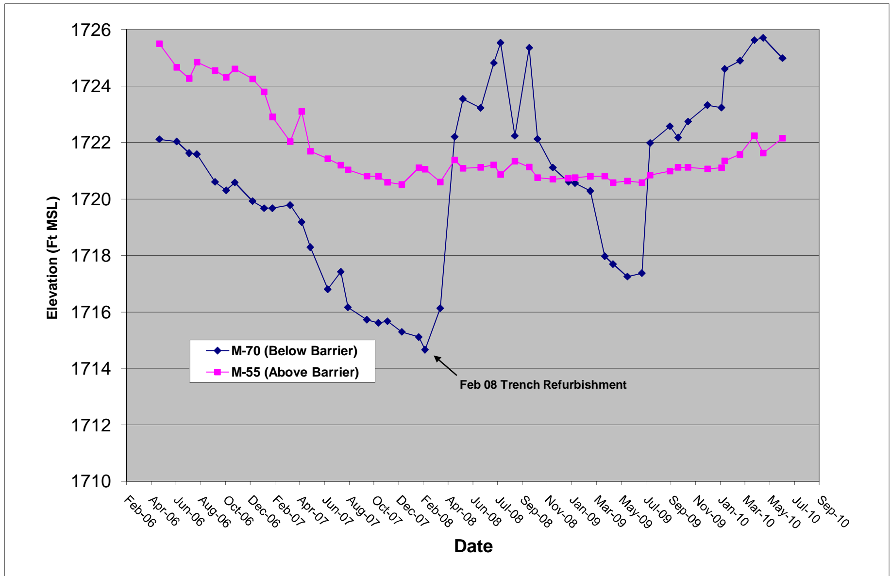
FIGURE 2 HYDROGRAPH PAIRS ACROSS THE BARRIER WALL
