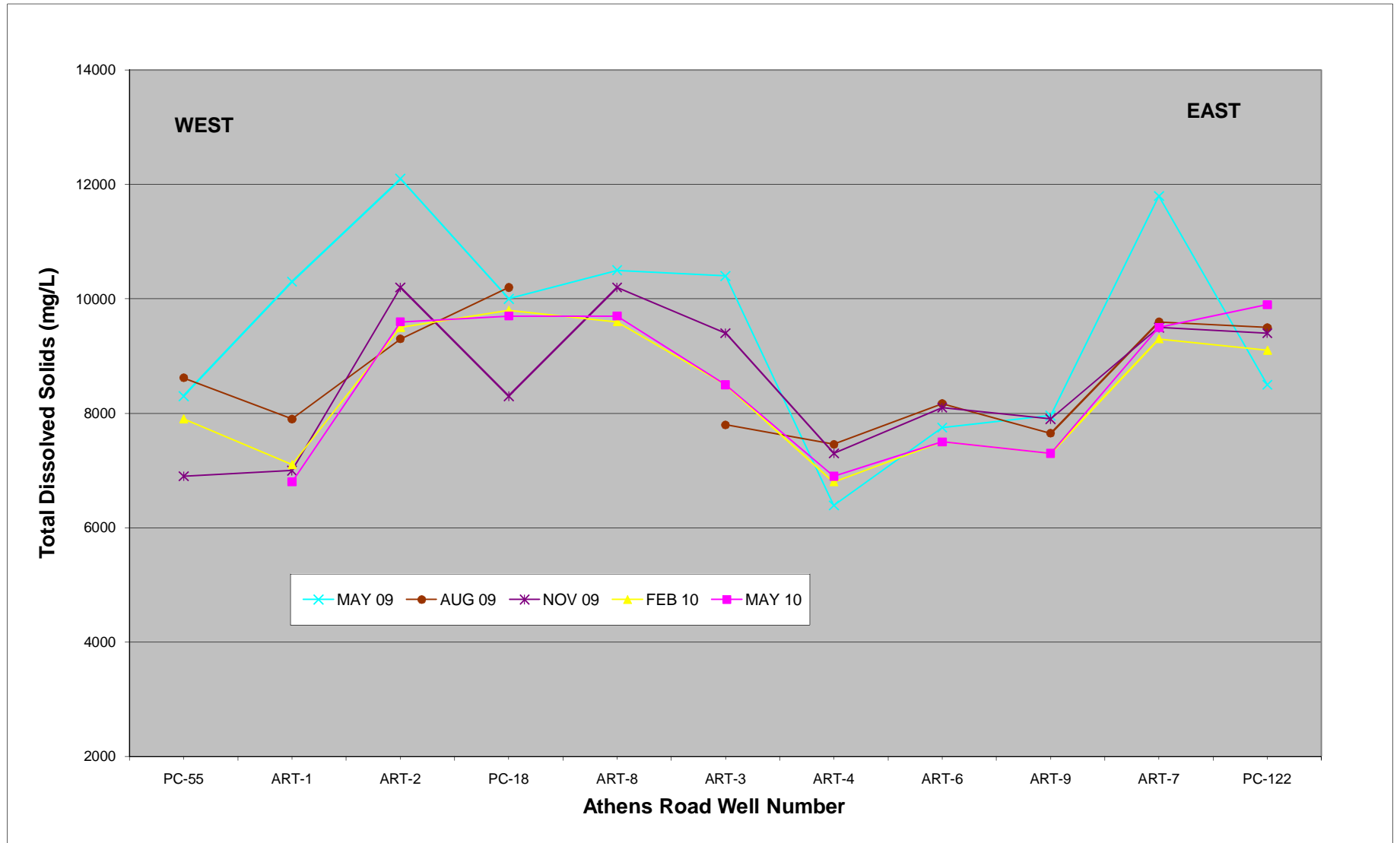
FIGURE 18 ATHENS ROAD WELL FIELD TOTAL DISSOLVED SOLIDS SECTION GRAPH
