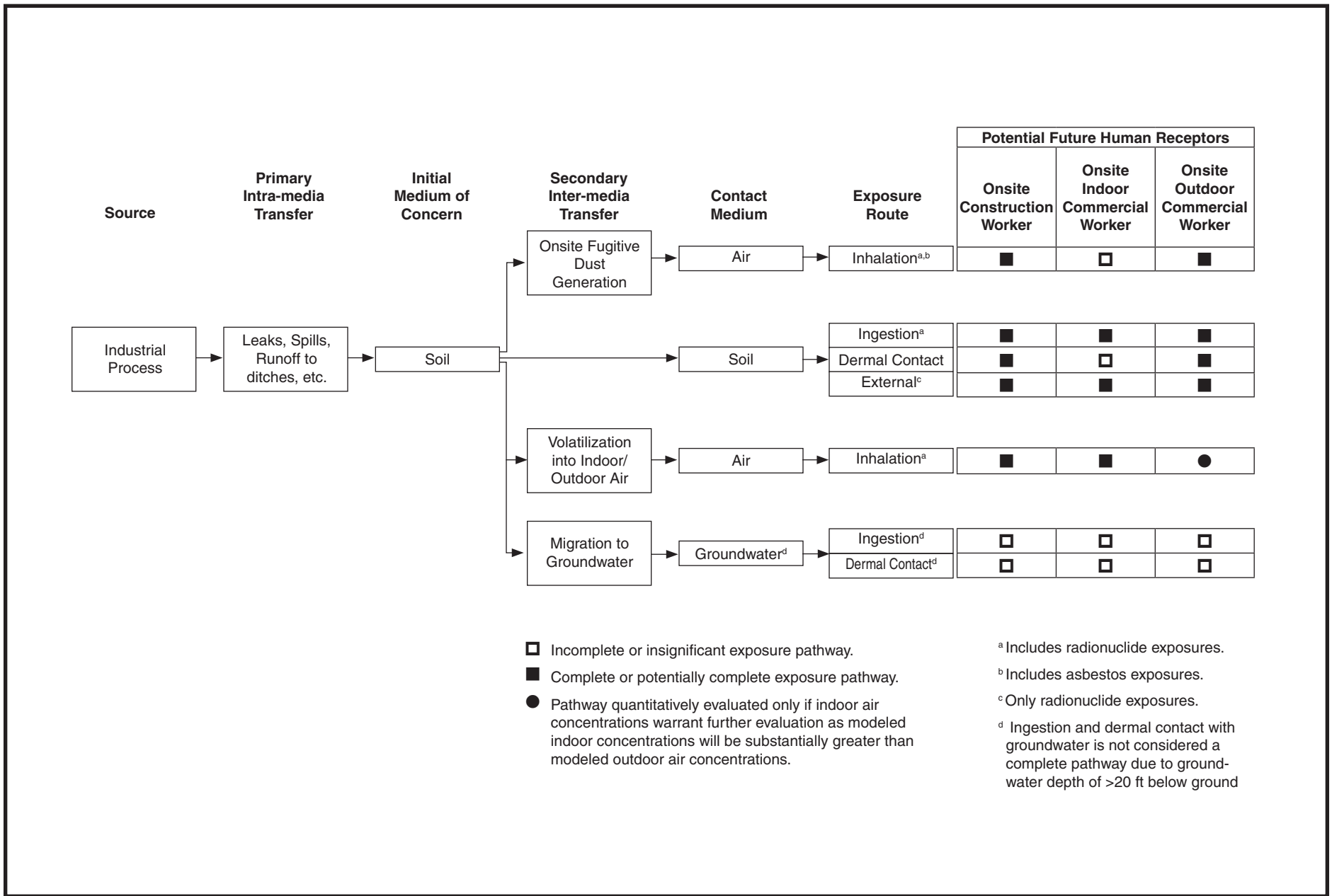
Figure 2. Conceptual site model diagram for potential human exposures—Tronox Facility, Henderson, Nevada
