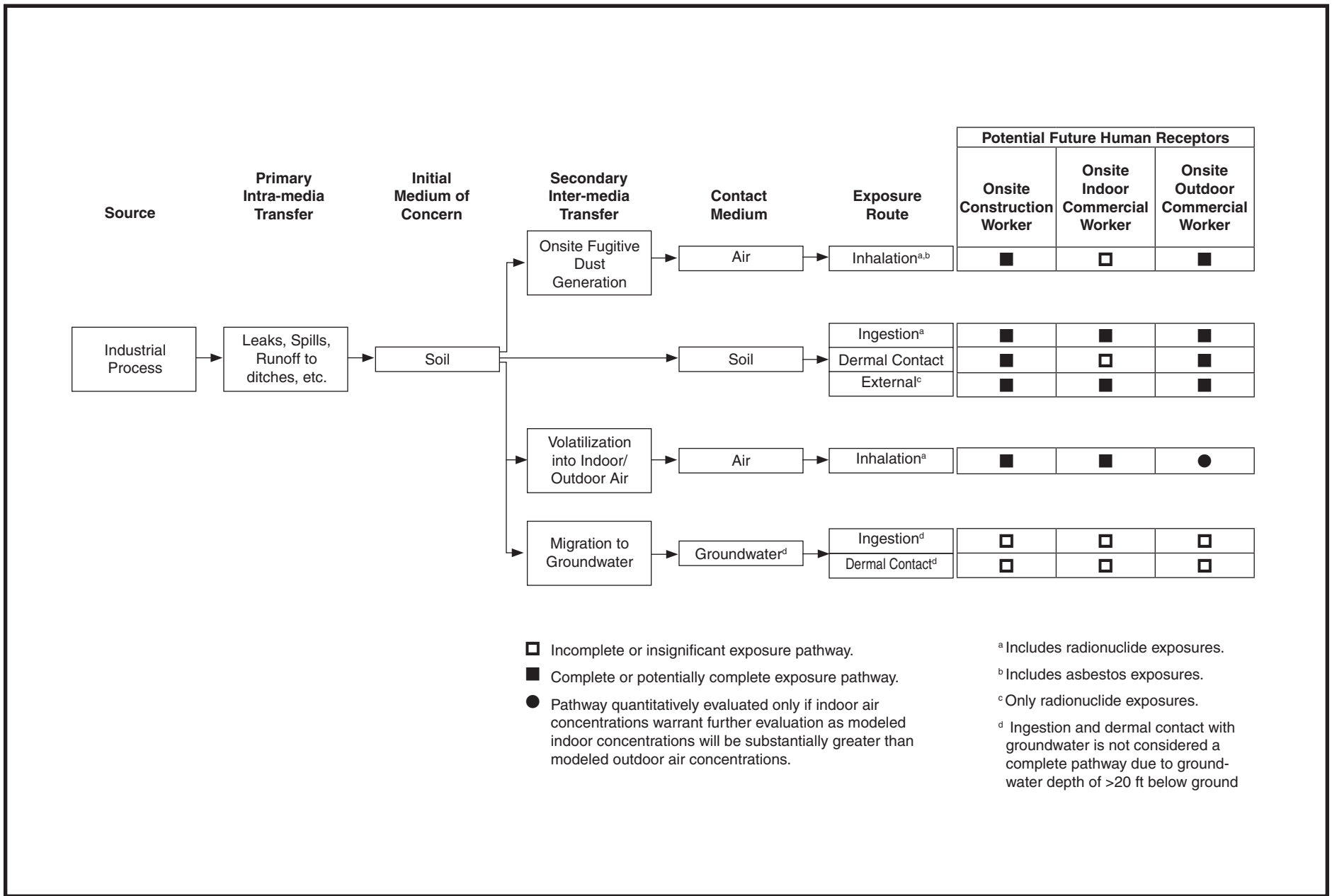
Figure 1. Conceptual site model diagram for potential human exposures—Tronox Facility, Henderson, Nevada
