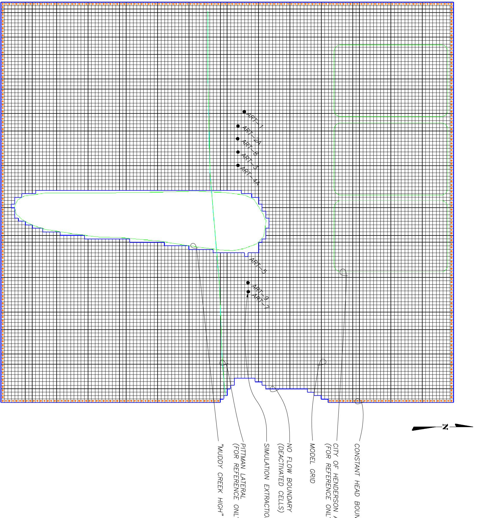
FIGURE 4 MODEL GRID AND BOUNDARY CONDITIONS
